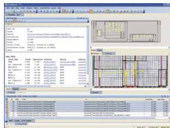
Figure 2 – Design connectivity in the schematic view and timing analysis with the larger components placed
