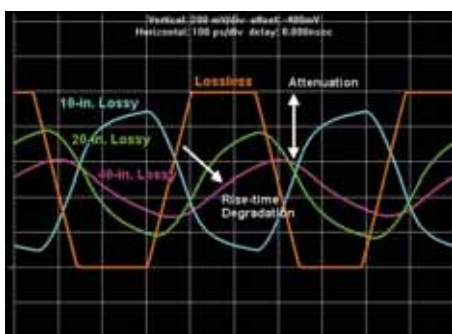
Figure 1 – Receiver waveforms for a lossless line, as well as 10, 20, and 40 in lines, showing both attenuation and rise-time degradation for a 2 GHz signal. (Simulated with Mentor Graphics HyperLynx.)
