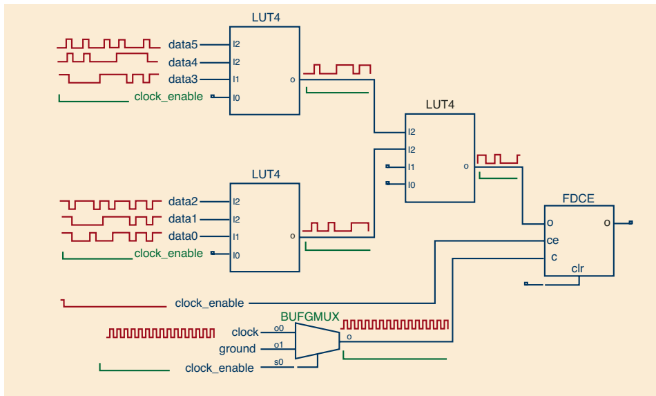
Figure 1 – Reducing power with enable signals
