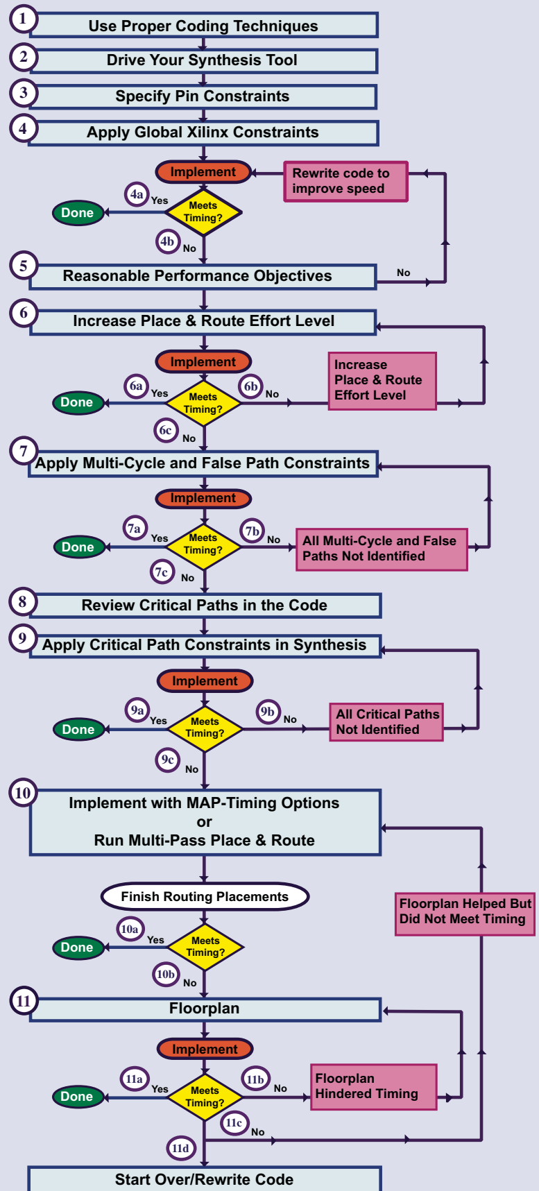
Figure 1 – Timing closure flow chart
