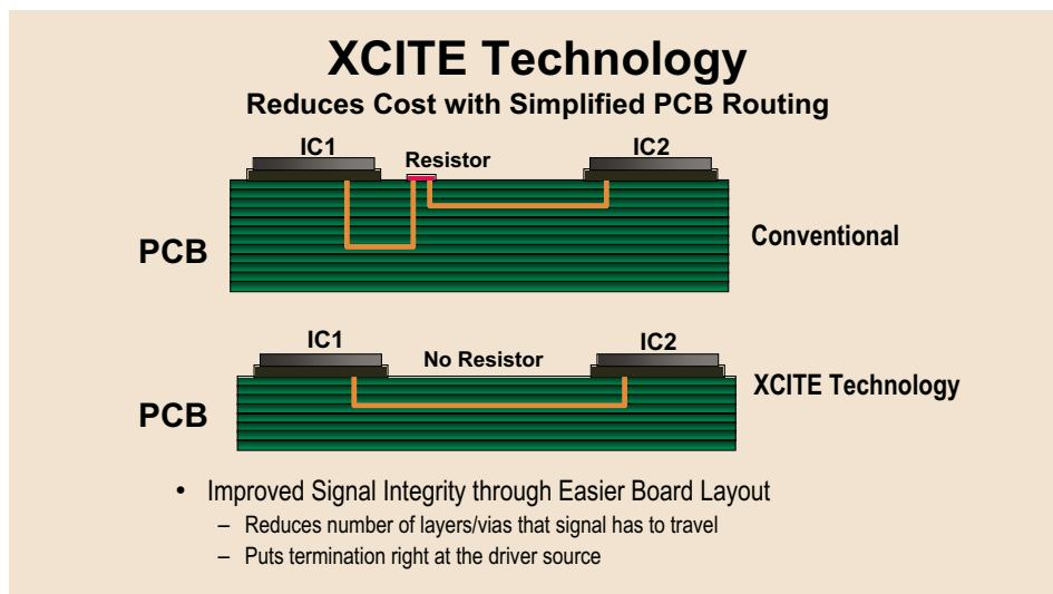
Figure 3 – Xilinx XCITE technology reduces cost through simplified PCB routing.
