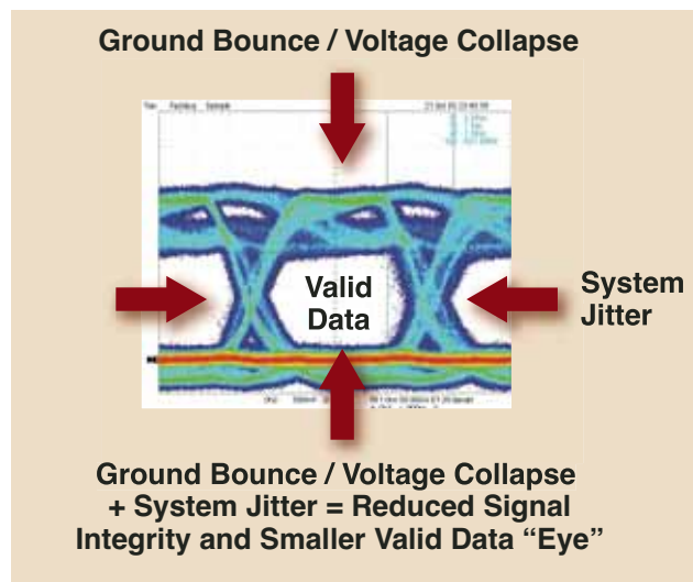
Figure 1 – How noise and jitter can affect an eye diagram.
