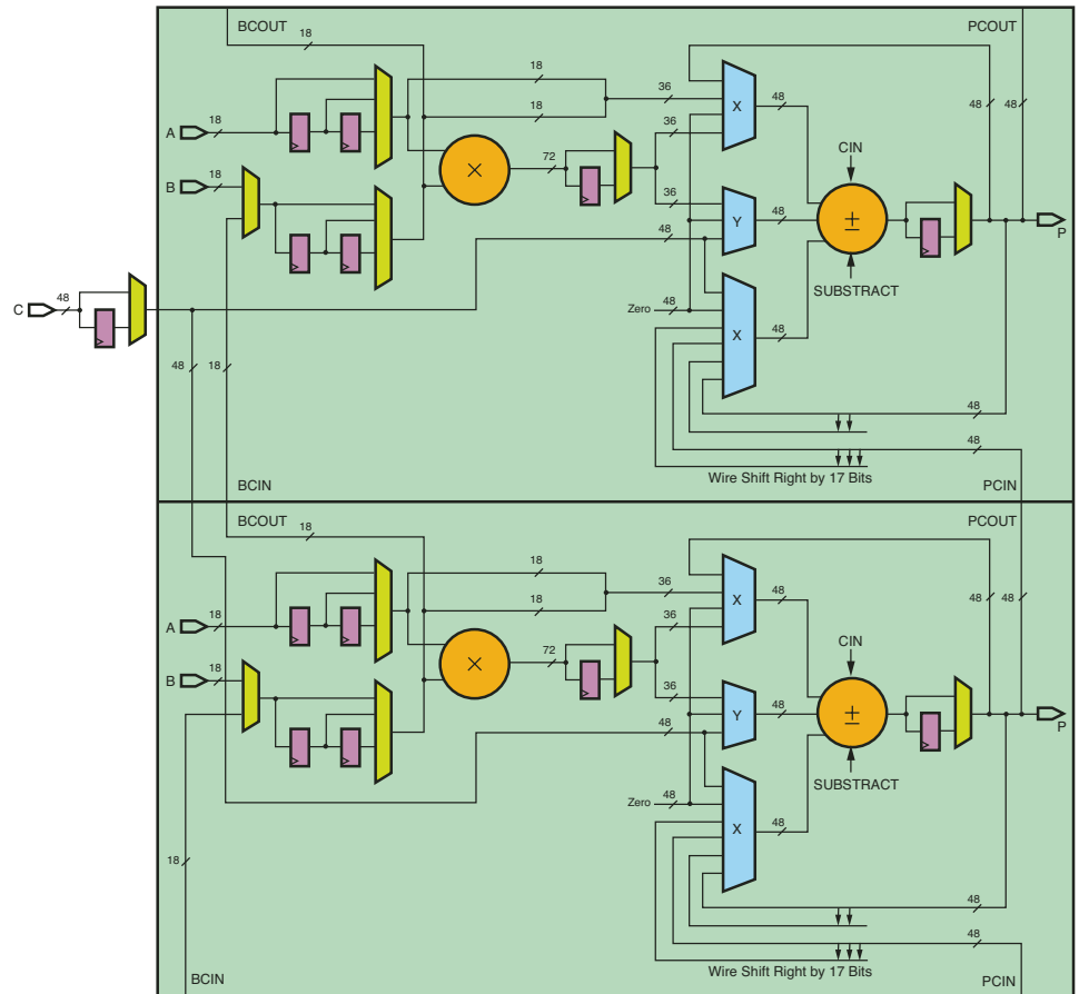
Figure 1 – DSP tile comprising two DSP48 slices
