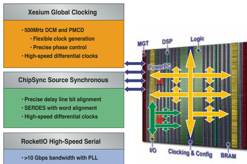
Figure 5 – Xesium clocking resources
