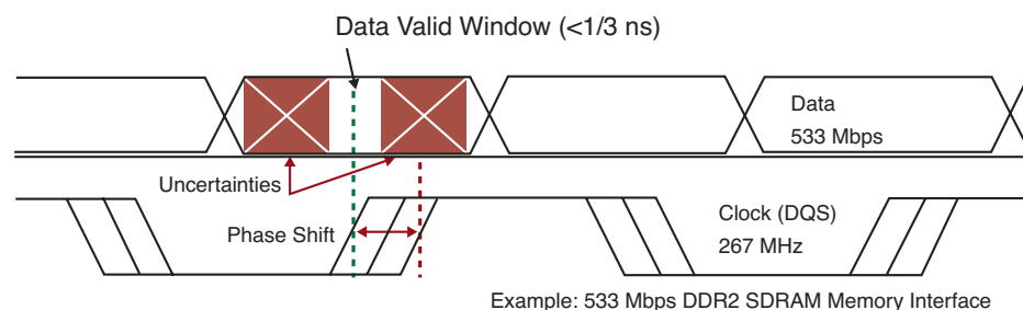
Figure 4 – Data valid window for a 533 Mbps DDR2 SDRAM interface
