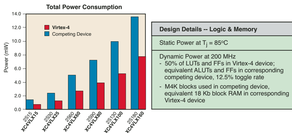
Figure 3 – Virtex-4 designs consume 1 to 5 watts lower power per FPGA
