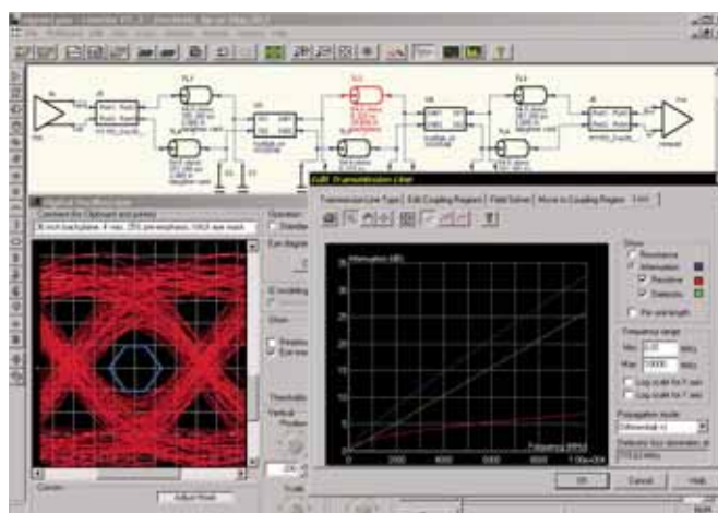
Figure 3 – Results with pre-emphasis bumped to 25% show significant improvement. Also shown is a graph of resistive and dielectric loss (dB) as a function of frequency (MHz) for the backplane (simulated with HyperLynx LineSim GHz).
