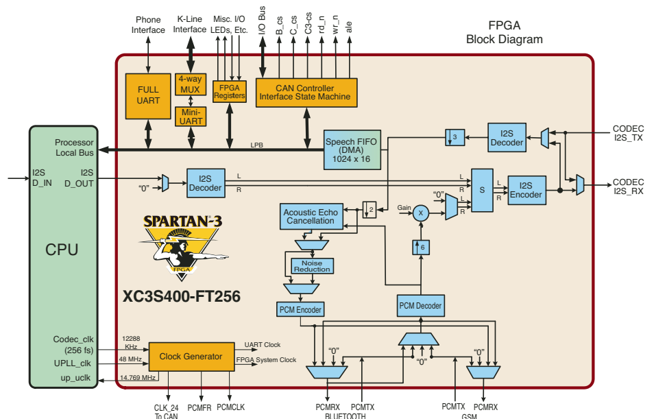
Figure 2 – Xilinx Spartan-3 FPGA design
