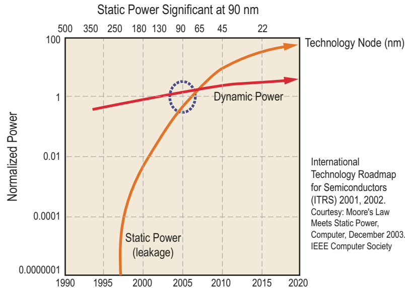
Figure 1 – The 90 nm inflection point
