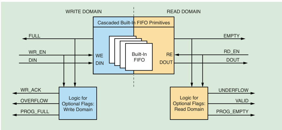
Figure 2 – Built-in FIFO capabilities expanded by the FIFO Generator
