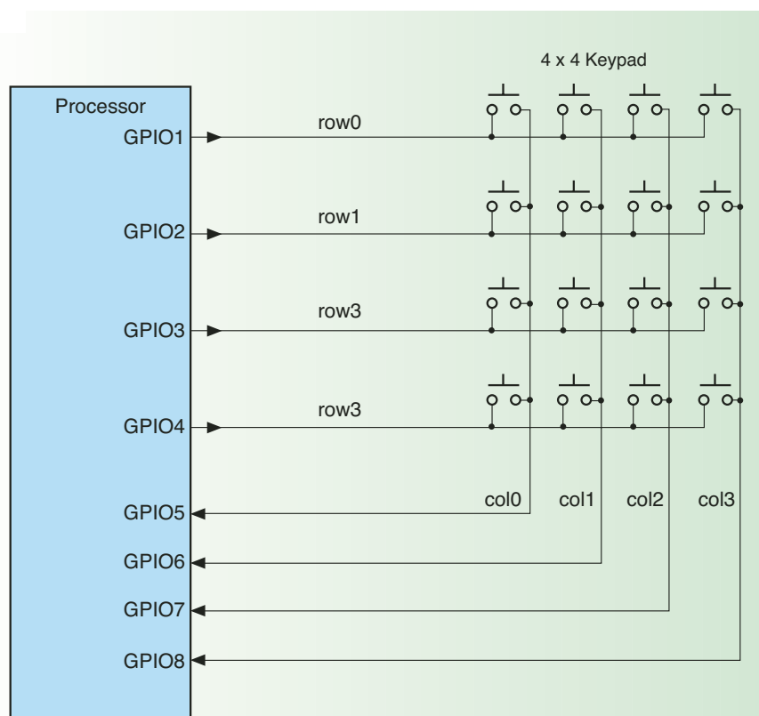
Figure 2 – Simple 4 x 4 keypad connected to a processor requiring eight GPIO
