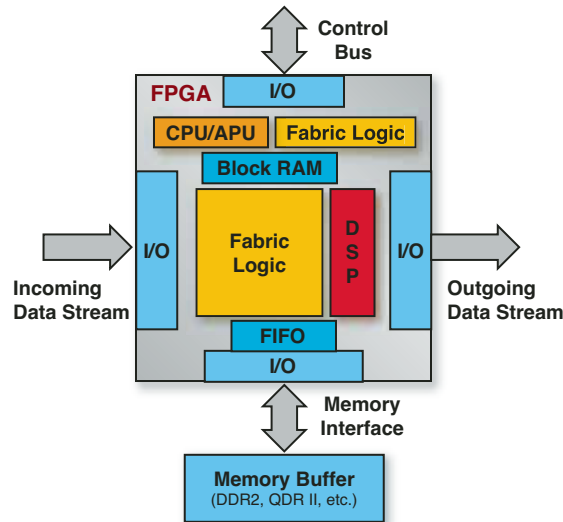
Figure 1 – FPGA-based system
