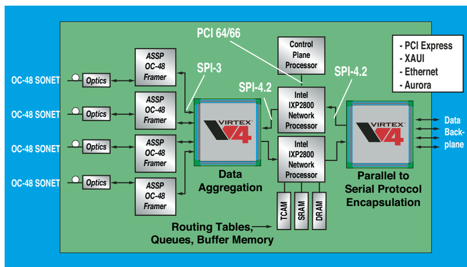
Figure 1 – Xilinx line-card example utilizing Virtex-4 FPGAs
