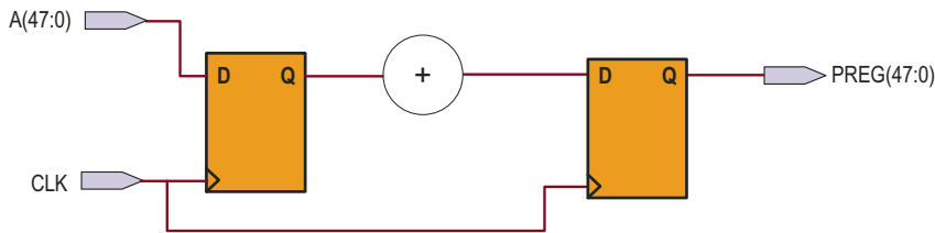
Figure 6 – RTL schematic for a simple INCDEC design
