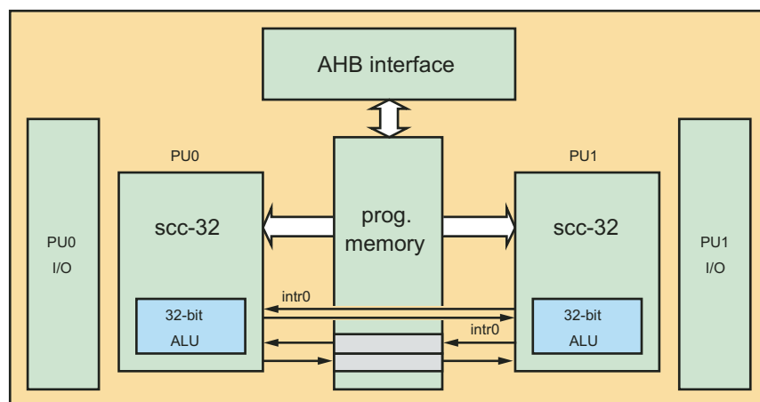
Figure 5 – Multiprocessor scheme with the scc-32
