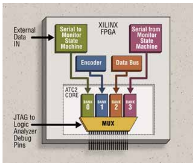
Figure 2 – ATC2 cores, inserted using the ChipScope Pro tool, allow you to quickly switch which signals are connected to pins for measurement. Each ATC2 core can be parameterized with as little as one signal bank or as many as 64 signal banks.
