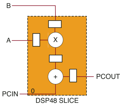
Figure 4 – A transposed MULT-ADD block diagram
