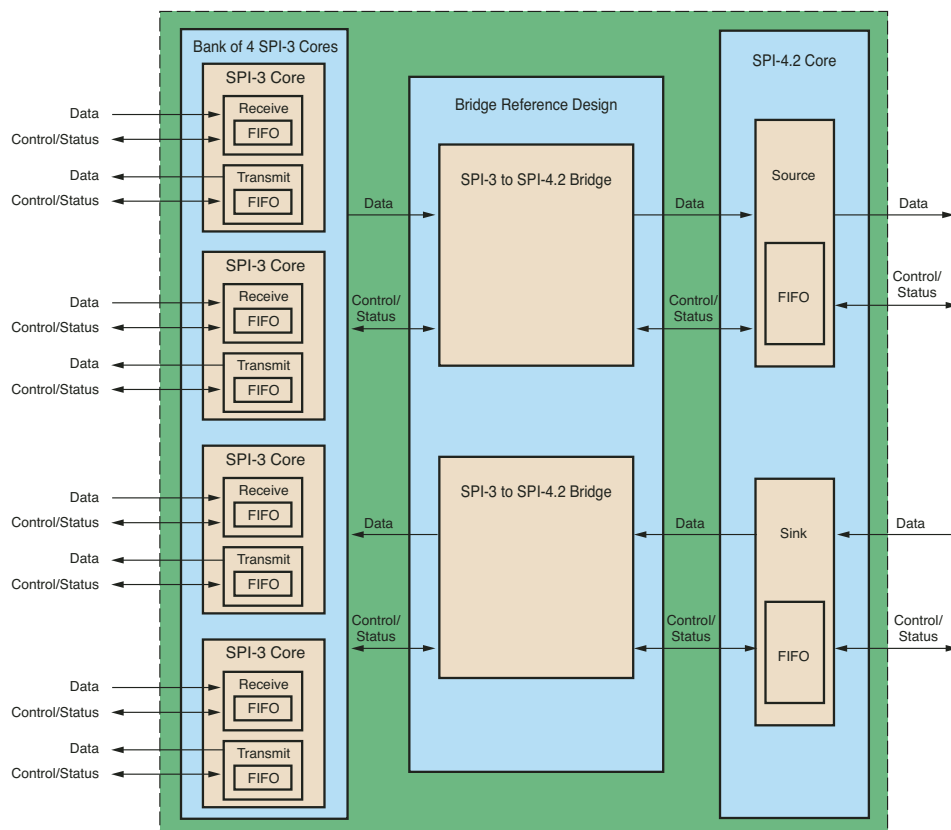
Figure 2 – Quad SPI-3 to SPI-4.2 bridge block diagram
