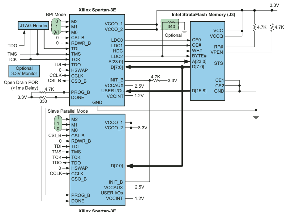
Figure 2 – A 2x Xilinx Spartan-3E FPGA to Intel StrataFlash memory (J3) connection (B4981)
