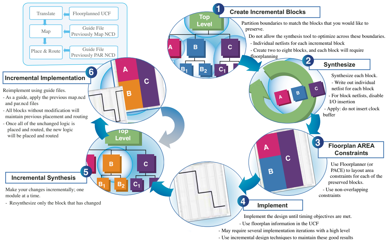
Figure 3 – Incremental design techniques/design flow
