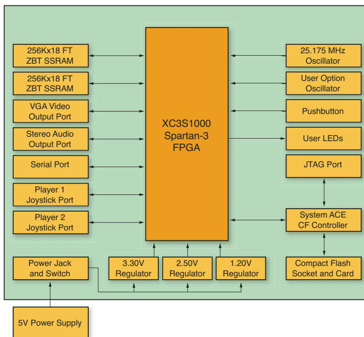
Figure 1 – Block diagram of a reconfigurable video game platform
