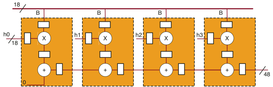
Figure 2 – A transposed FIR filter block diagram
