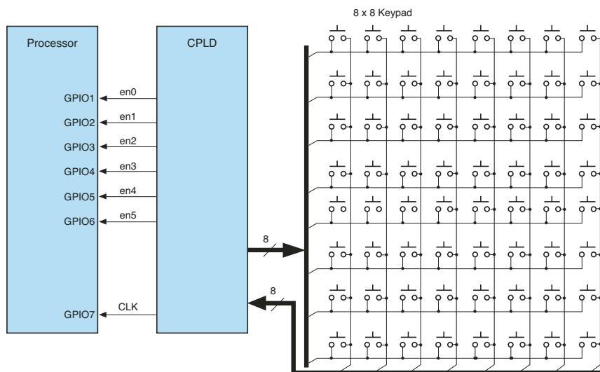
Figure 3 – GPIO expansion with a CoolRunner-II CPLD
