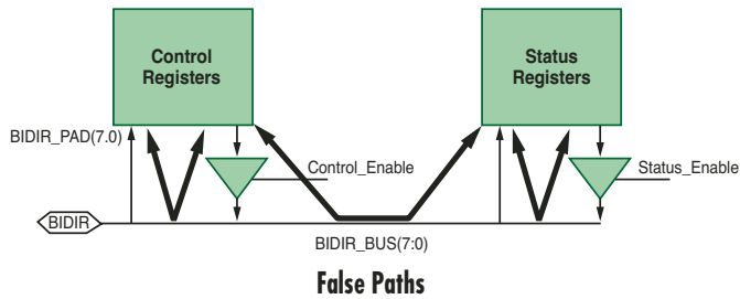
Figure 2 – False paths through bi-directional pad
