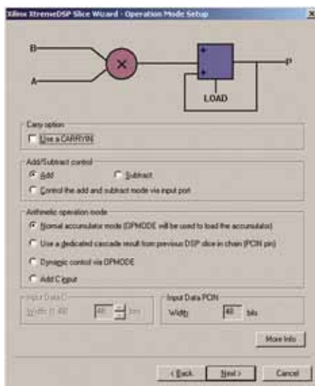
Figure 1 – XtremeDSP architecture wizard
