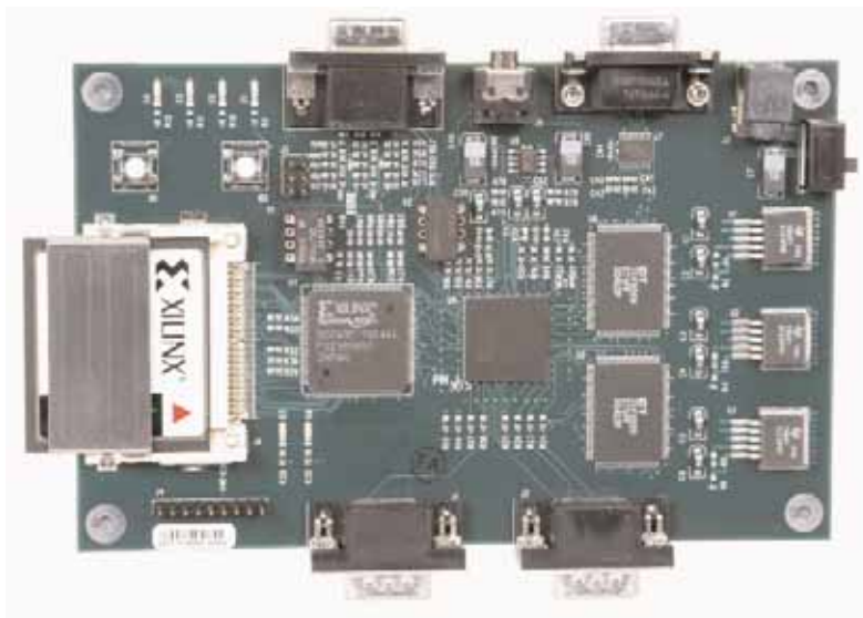
Figure 2 – Prototype of a reconfigurable video game platform
