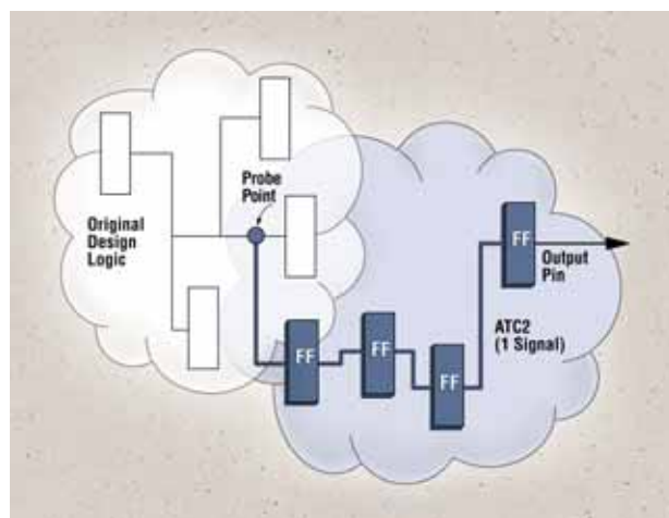
Figure 3 – A pipelined architecture uses four stages to route a signal to the debug port using the FPGA Dynamic Probe. This automated approach gives the place and route tool flexibility to meet timing requirements because the router can use timing solely within the ATC2 core to move across the chips.
