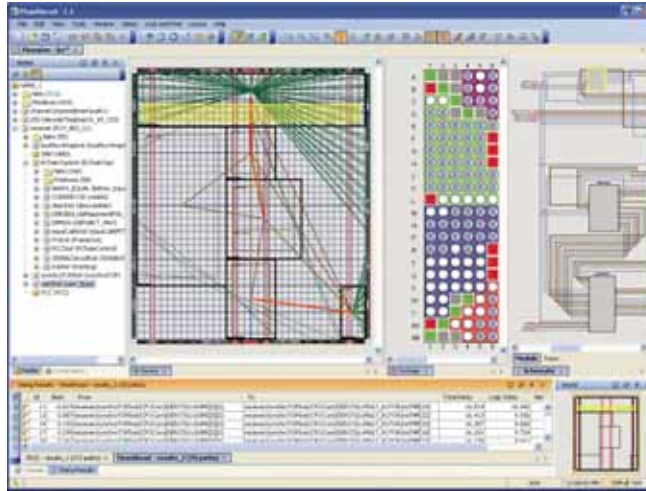
Figure 3 – The device, package, and schematic views of the design with timing analysis from TimeAhead
