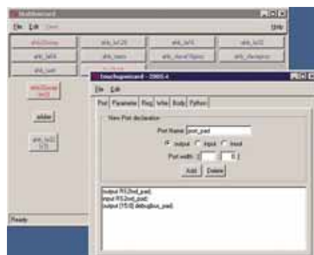
Figure 4 – AHBWIZARD with touch-up wizard screen shot
