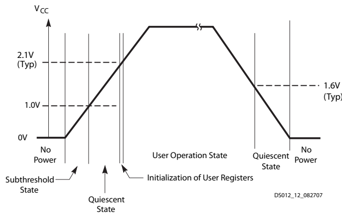
Figure 3: Device Behavior During Power Up
