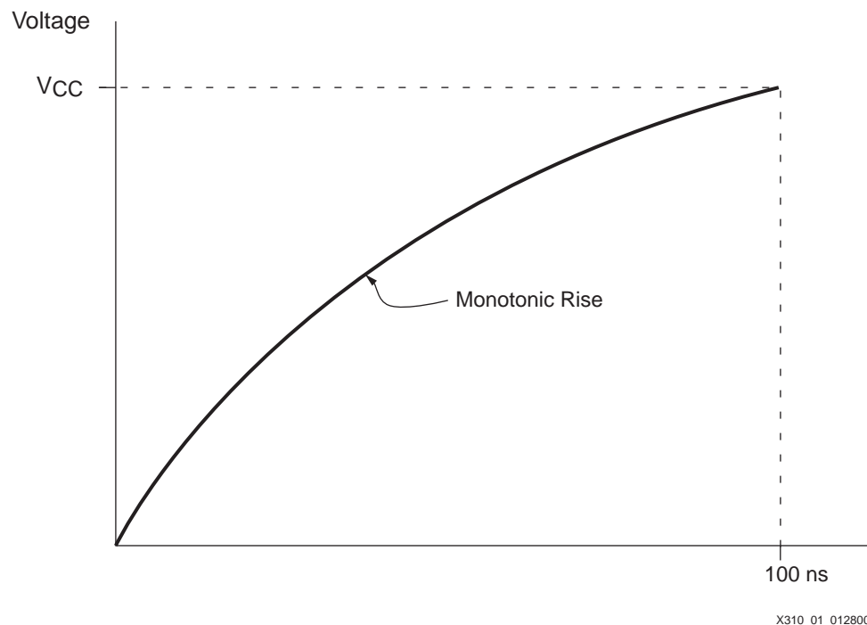
Figure 1: "Ideal" Voltage Ramp
