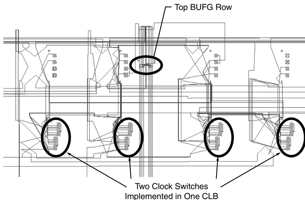
Figure 9: Placement of Clock Switch as Shown in FPGA Editor
