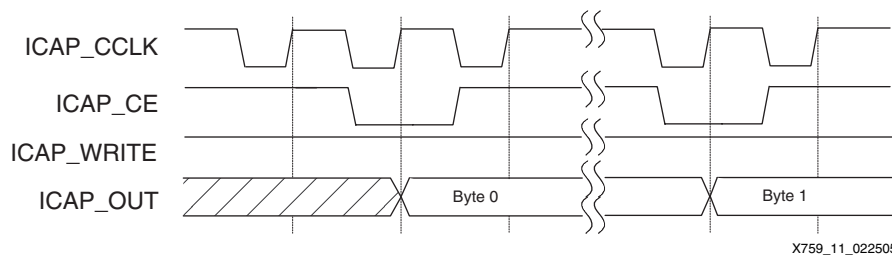
Figure 11: ICAP Read Timing with Controlled ICAP Clocking
