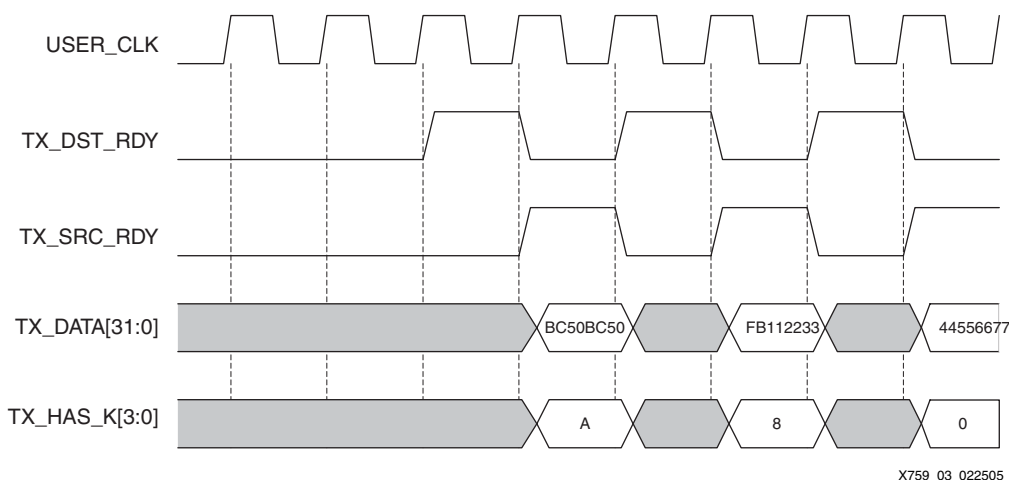
Figure 3: Frame Transmission on Transparent Mode Client Interface
