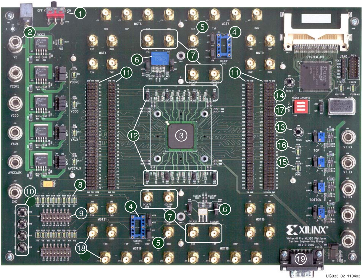
Figure 2: Detailed Description of Virtex-II Pro ML32x Platform Components
