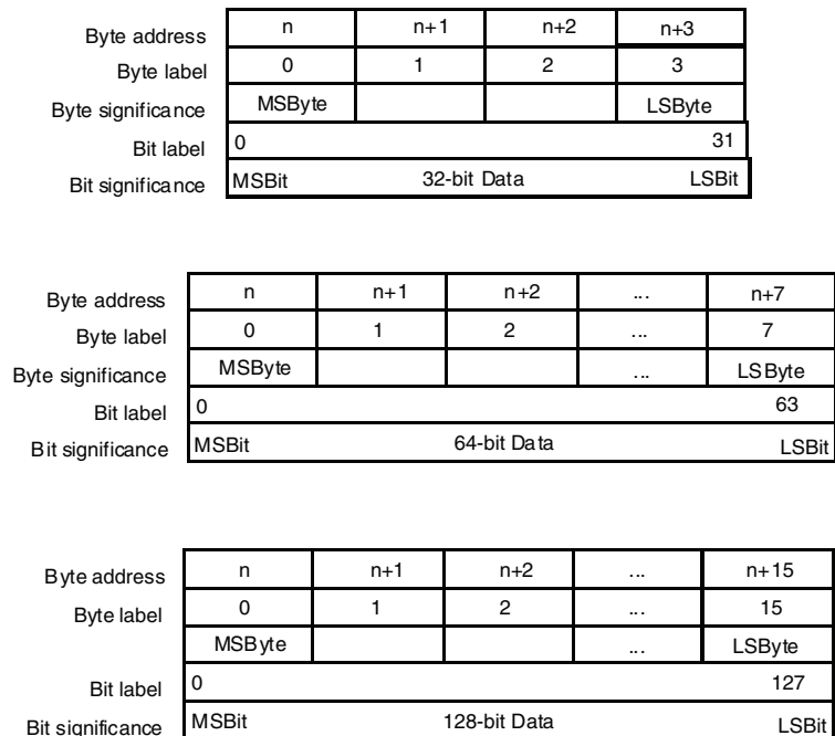
Figure 2: Big-Endian Byte Ordering and Left to Right Bit Numbering
