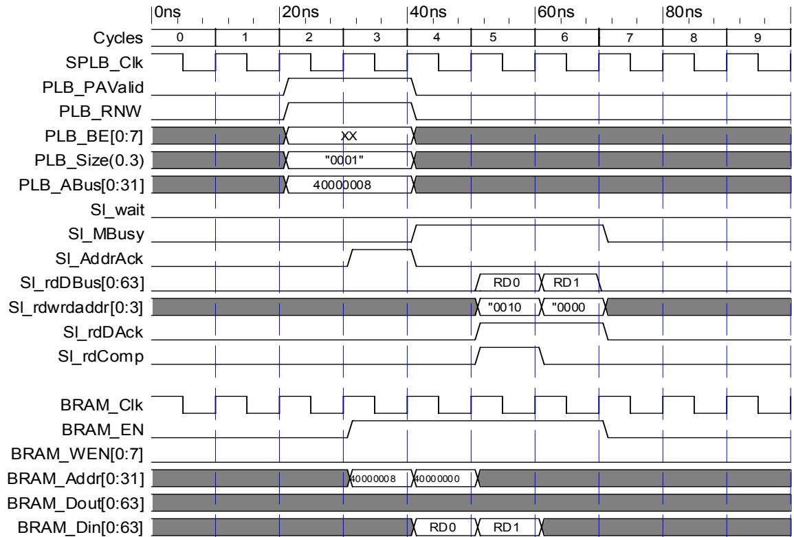
Figure 5: 4-Word Cacheline Read (C_SPLB_SUPPORT_BURSTS = 1)
