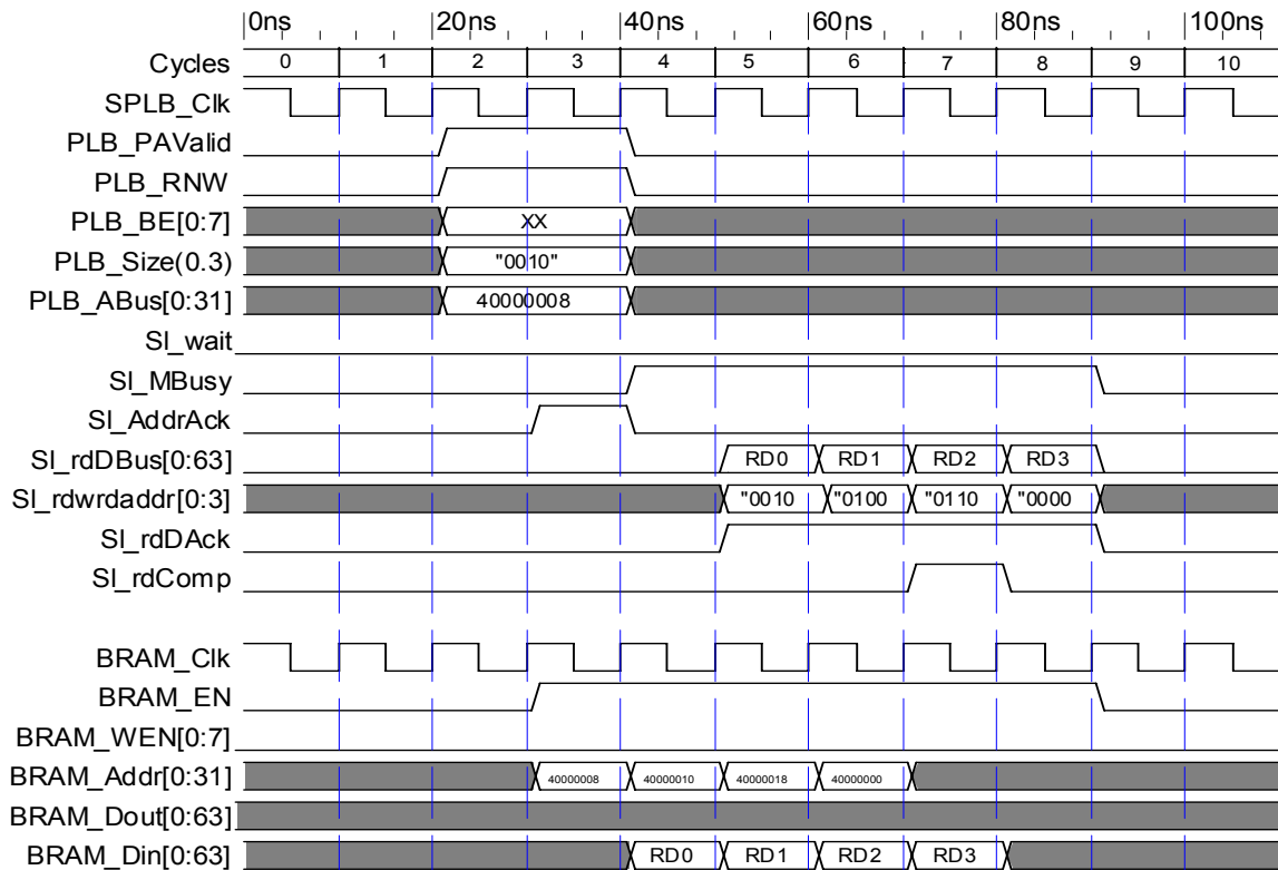
Figure 6: 8-Word Cacheline Read (C_SPLB_SUPPORT_BURSTS = 1)
