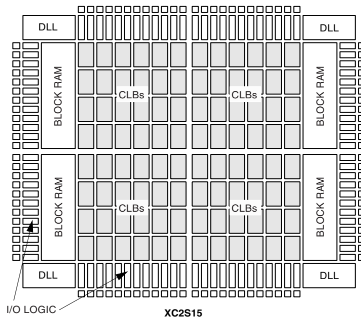
Figure 1: Architecture on Spartan-II FPGAs
