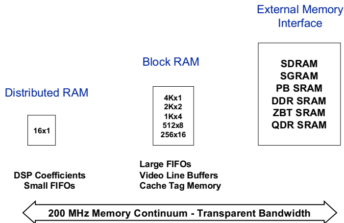
Figure 2: Embedded Memory Solutions from Xilinx Allow 200 MHz Memory Continuum Between Internal and External Memories
