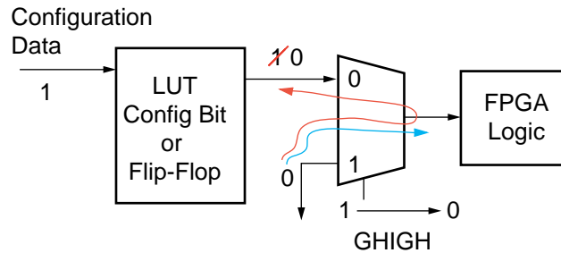
Figure 3: Incorrect FPGA Configuration Caused by Sensitivity to Process Corners
