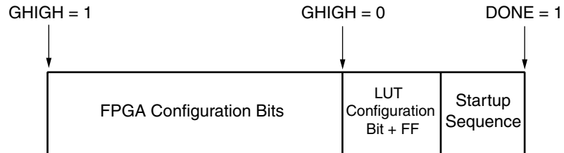
Figure 4: New Bitstream Configuration Methodology
