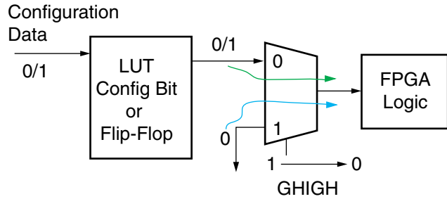
Figure 1: Normal Bitstream Loading Sequence
