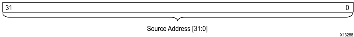
Figure 2-9: SA_MSB Register
