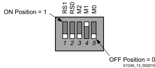
Figure 13: VC707 Board DIP Switch SW11
