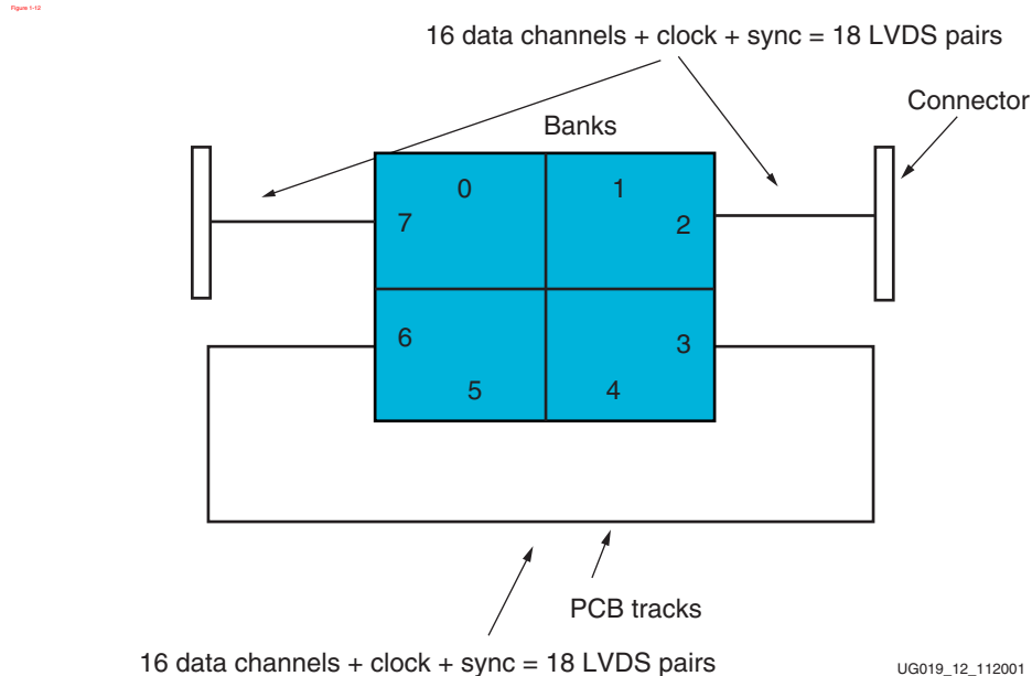
Figure 1-12: LVDS Interface Setup
