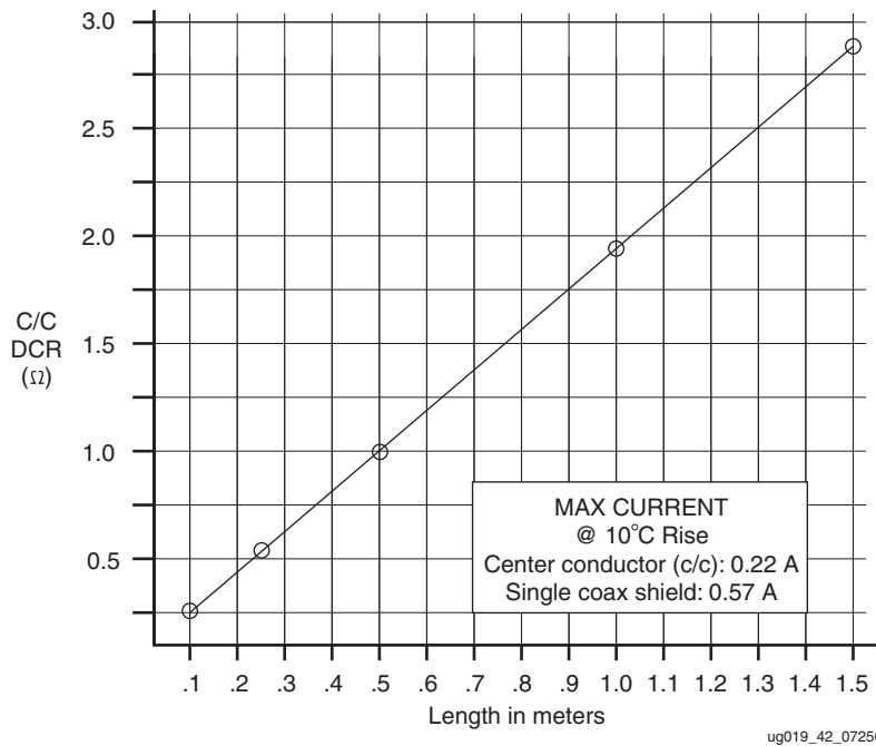
Figure 7-4: Typical DCR and Maximum Current-Carrying Capacity
