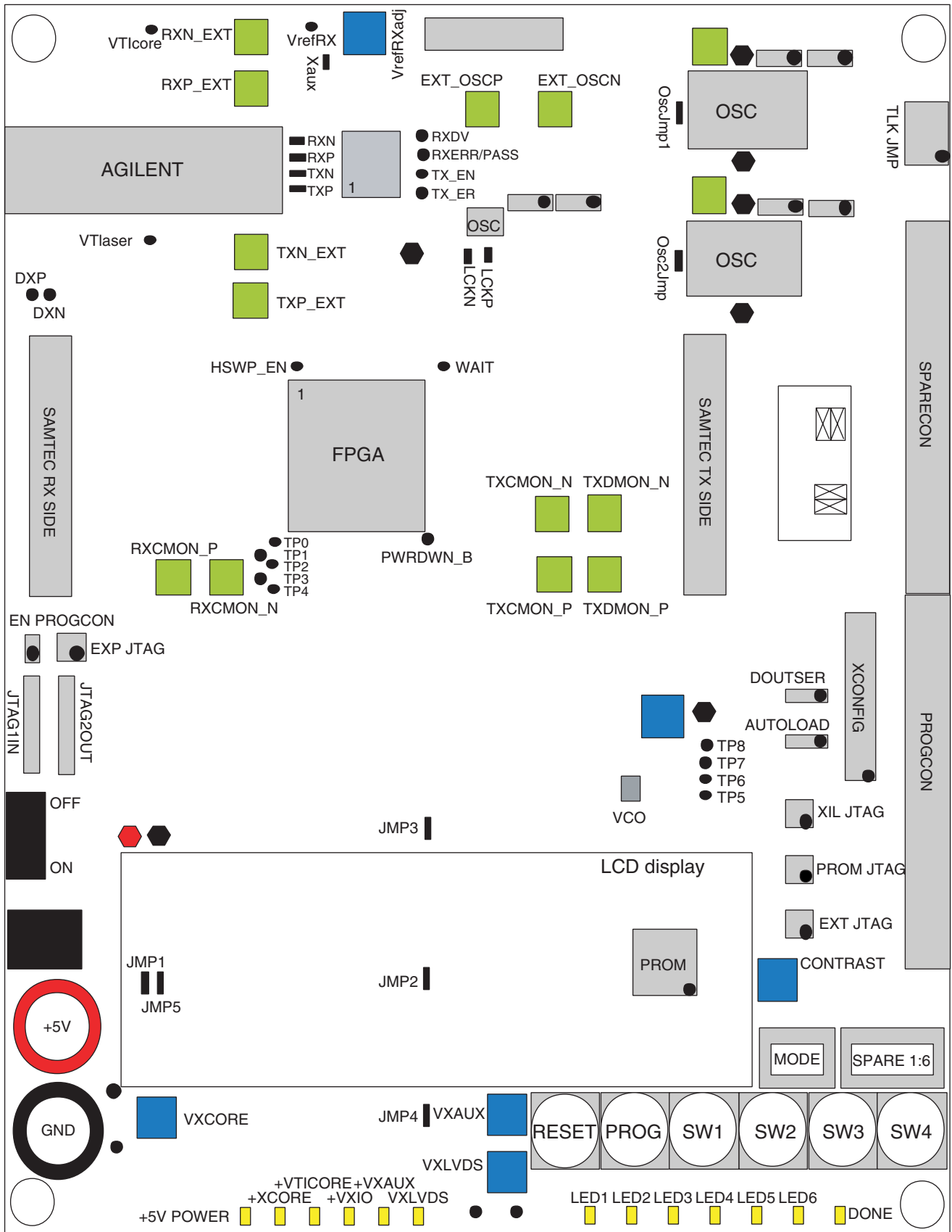
Figure 1-1: PCB Overview Drawing
