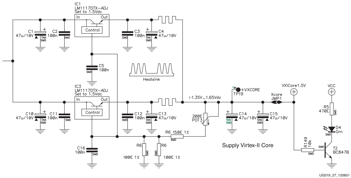
Figure 2-2: Power Supply 1.5
