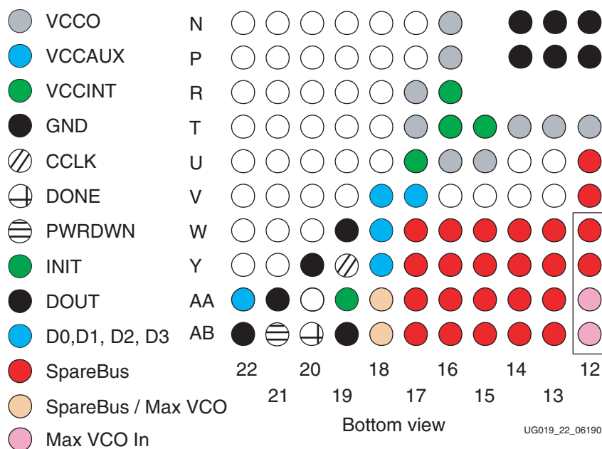
Figure 1-22: Bank 4 - SpareCon
