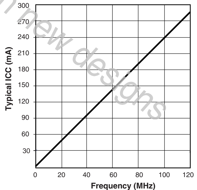
Figure 1: XCR3512XL Typical I_{CC} vs. Frequency at V_{CC} = 3.3\text{V} , 25^\circ\text{C}
