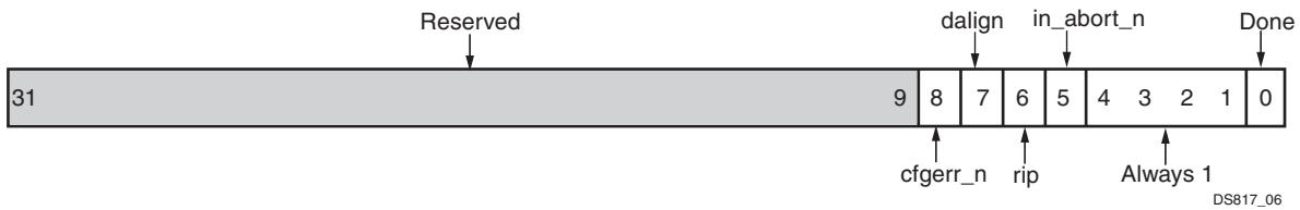
Figure 6: Status Register (SR)
