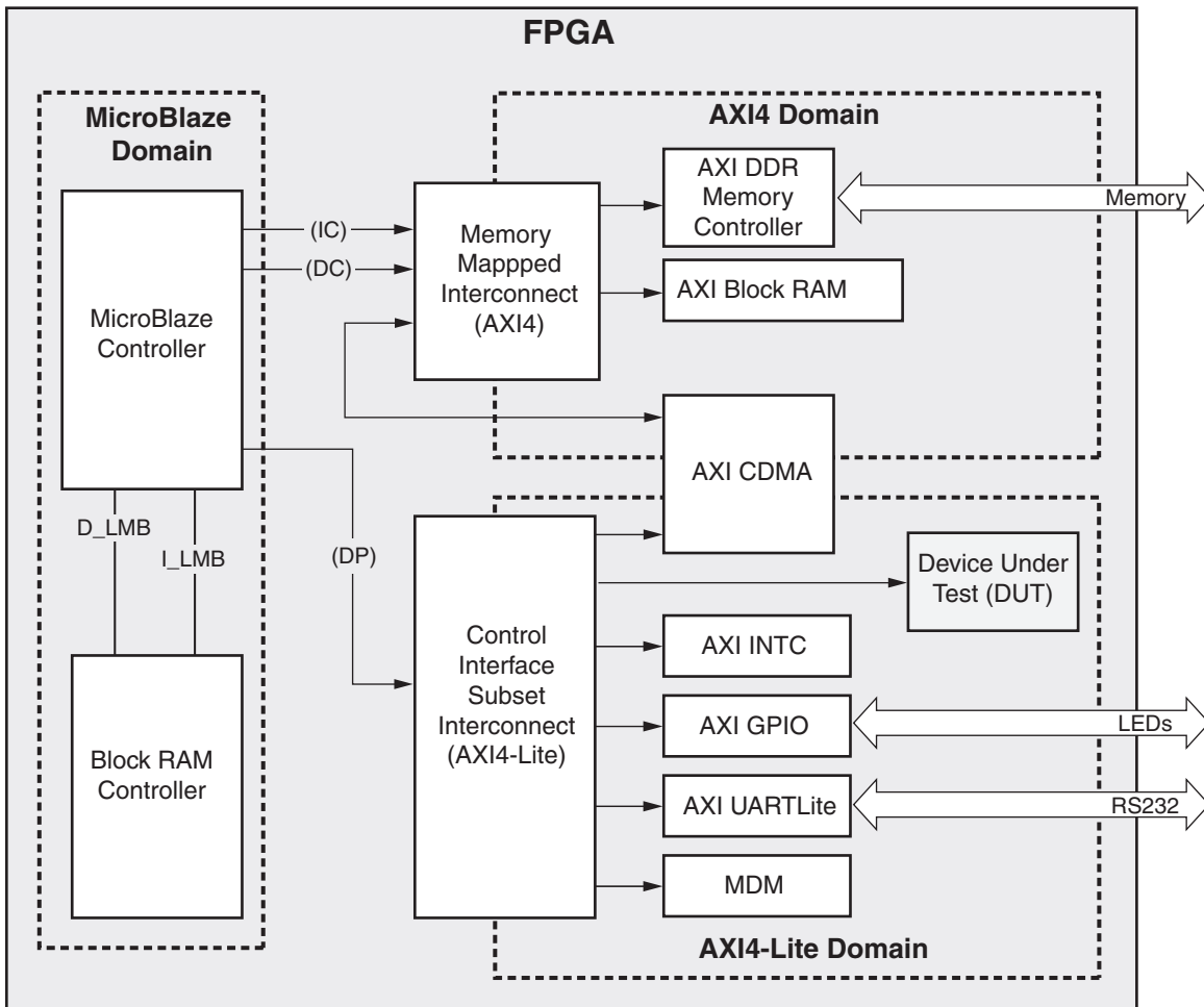
Figure 15: Virtex-6 and Spartan-6 FPGA System with the AXI HWICAP Core as the Device Under Test (DUT)
