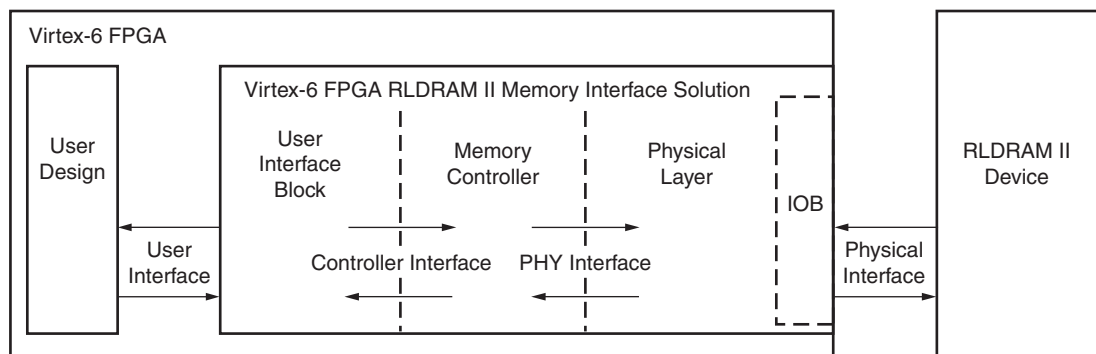
Figure 3: RLDRAM II Memory Interface Core
