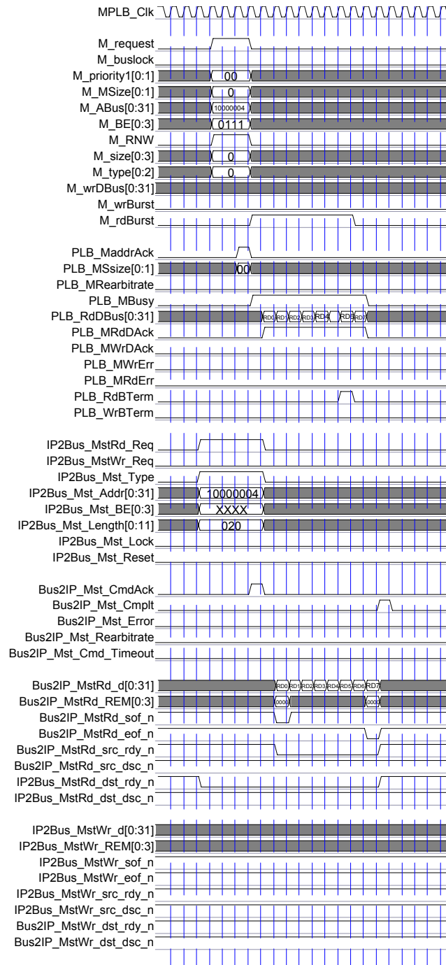
Figure 7: Fixed Length Burst Read Timing
