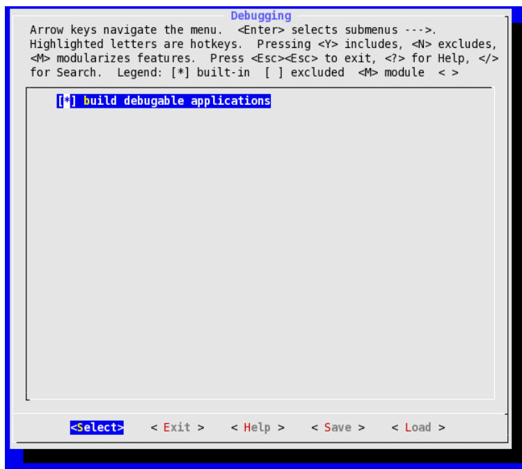
Figure 6: Debugging Menu
