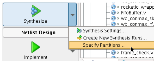
Figure 15: Specify Partitions
