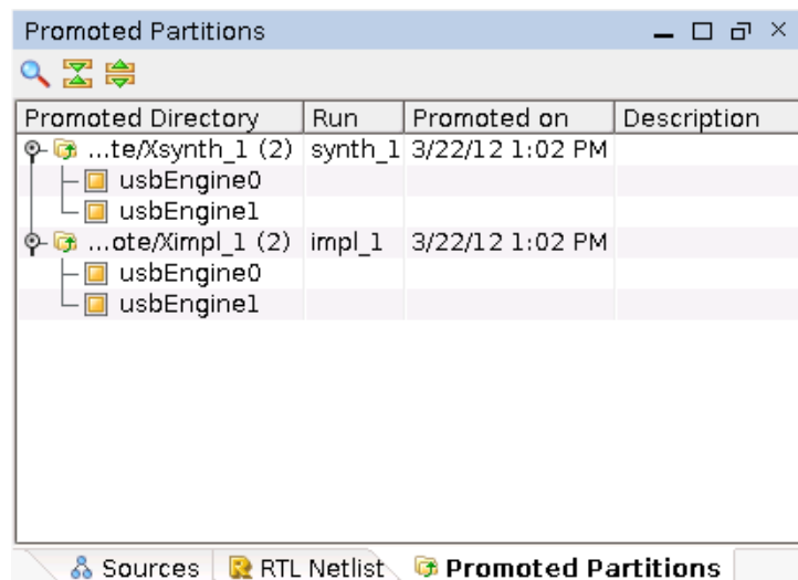
Figure 13: Promoted Partitions
