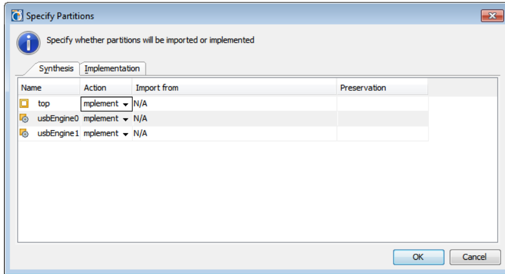
Figure 6: Specify Partitions
