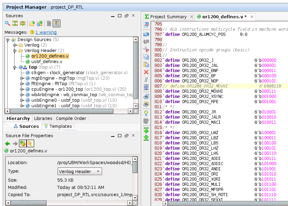
Figure 13: Updating or1200_defines.v
