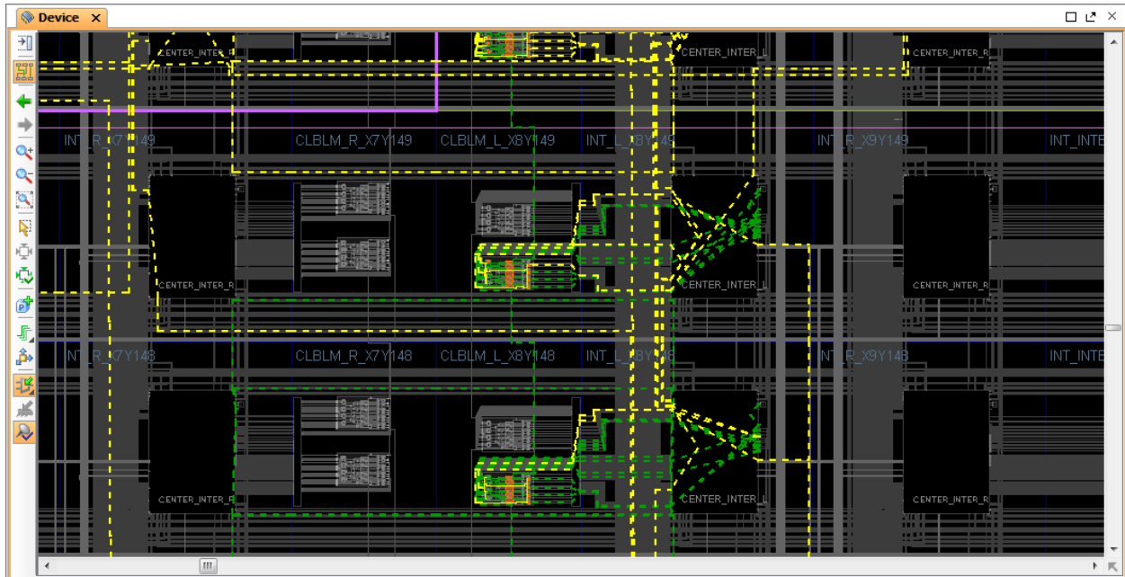
Figure 9: Closeup of Static-Only Design with Locked Routing
