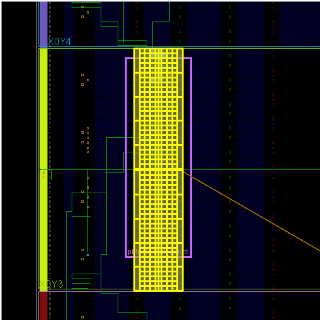
Figure 10: Reconfigurable Partition Frames Highlighted
