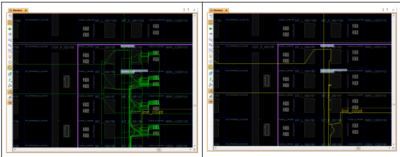
Figure 8: The inst_count module before (left) and after (right) update_design -black_box
