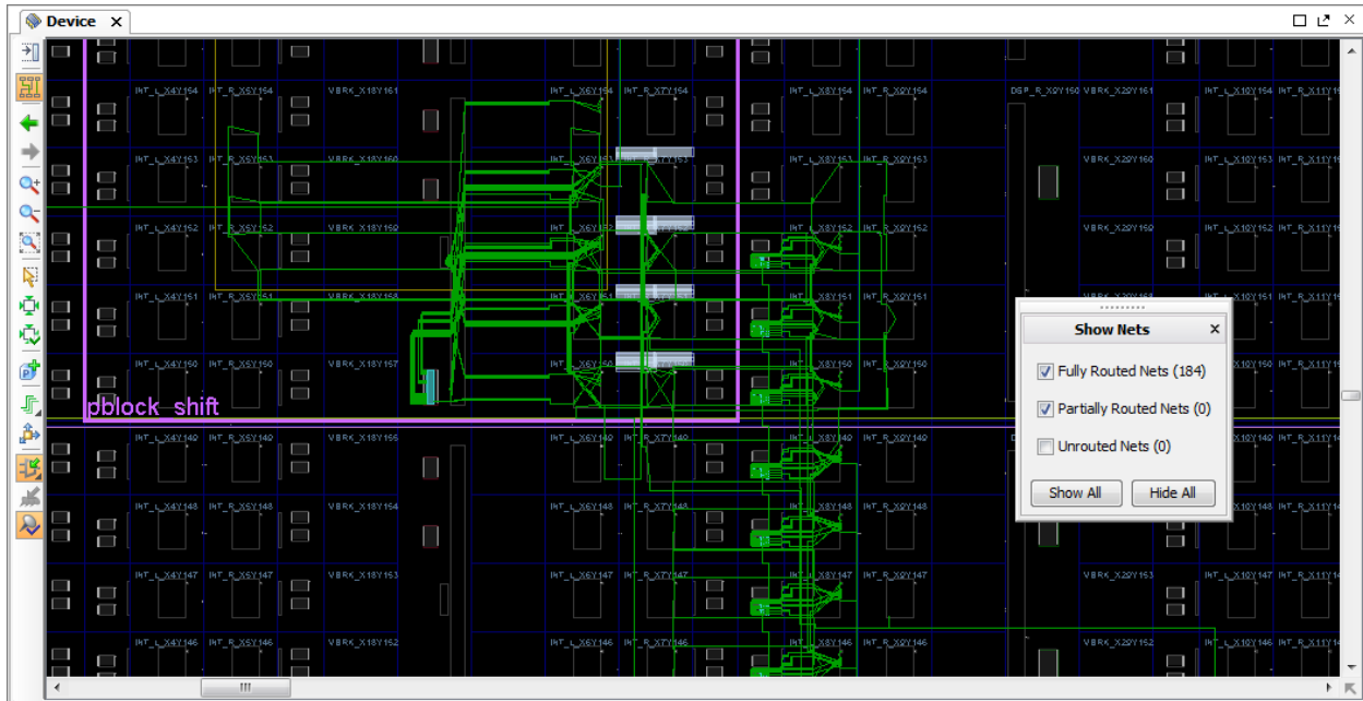
Figure 7: Closeup of First Configuration Routed
