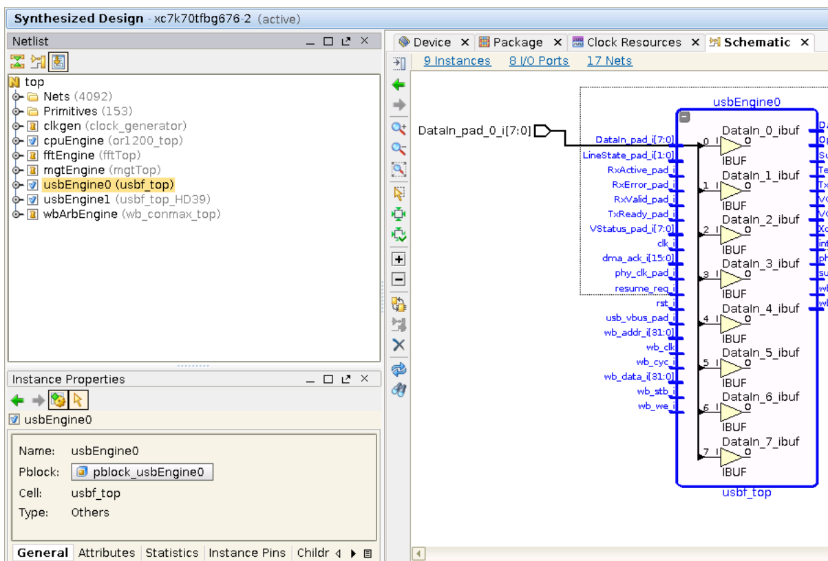
Figure 1: Schematic View
