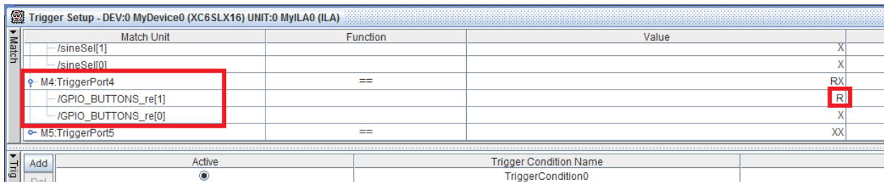
Figure 12: Changing the trigger condition of GPIO_BUTTONS_re[1]
