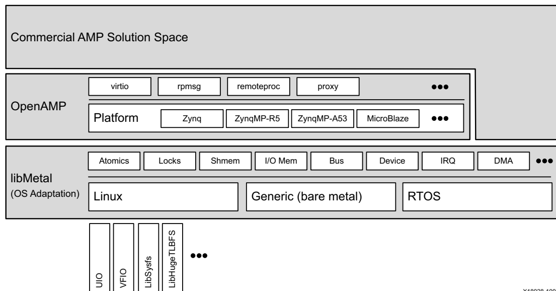
Figure B-1: OpenAMP libmetal Architecture
