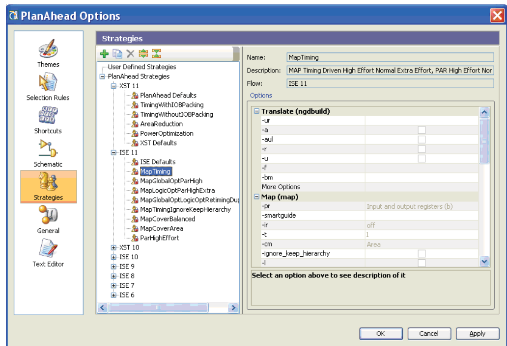
Figure 1: PlanAhead Tool Strategies
