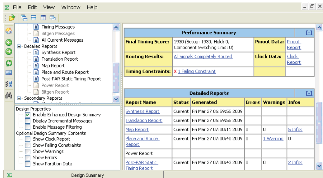
Figure 6: Project Navigator Reports
