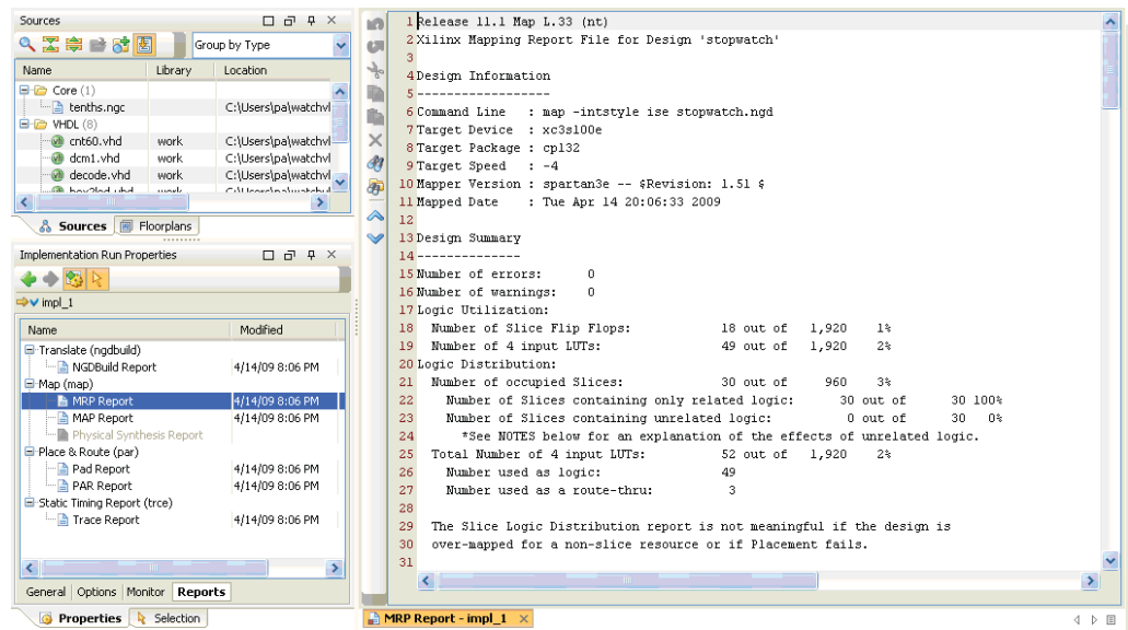
Figure 5: PlanAhead Tool Implementation Run Reports
