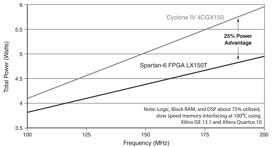
Figure 7: Total Power Consumption Comparison
