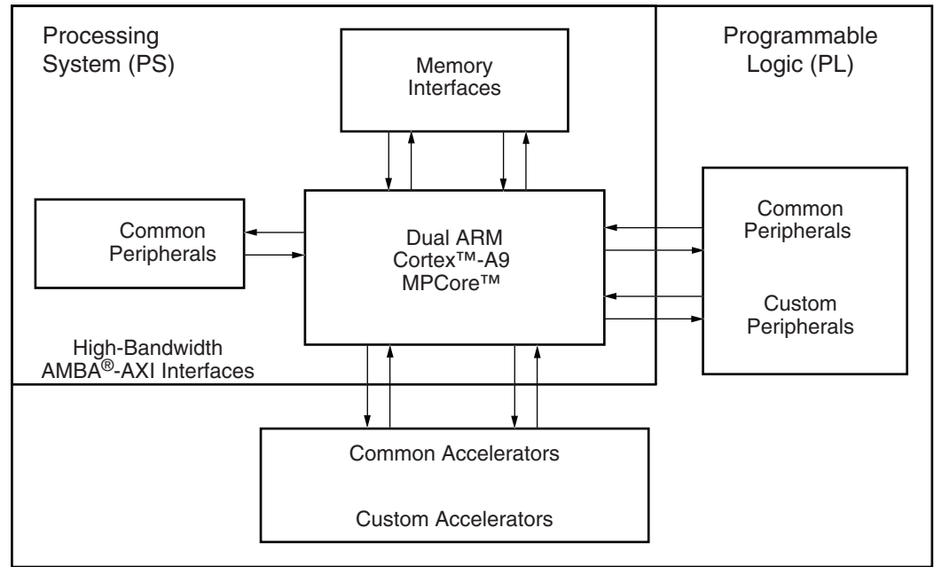
Figure 6: Zynq-7000 EPP
