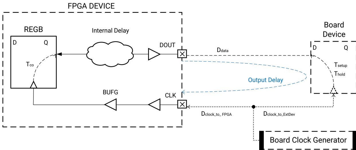
Figure 95: Output Delay Computation
