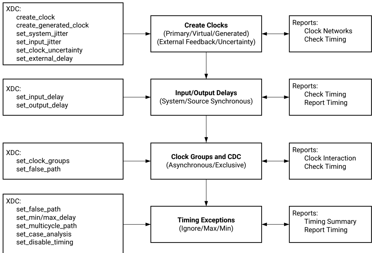
Figure 87: Steps for Developing Timing Constraints
