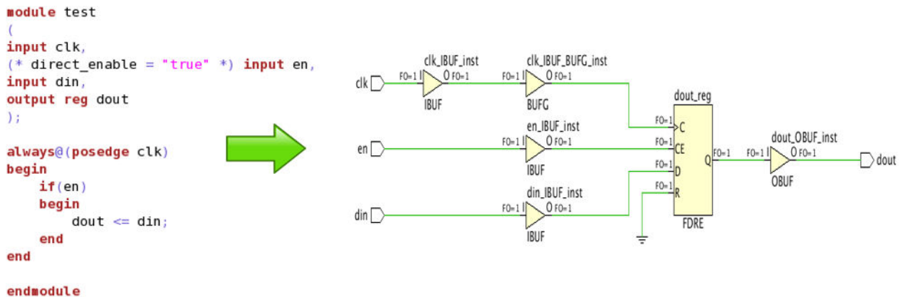
Figure 23: Dedicated Clock Enable Implementation Using direct_enable
