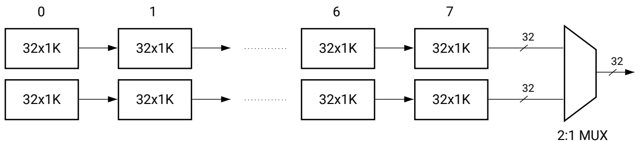
Figure 45: Generated Structure for 32x16K Memory Configuration Using the RAM_DECOMP Attribute
