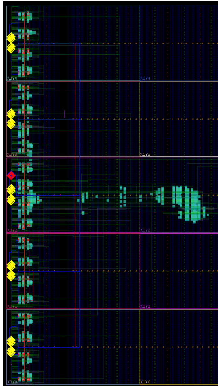
Figure 77: TXUSRCLK/TXUSRCLK2 Clock Routing for a Multi-Quad Interface
