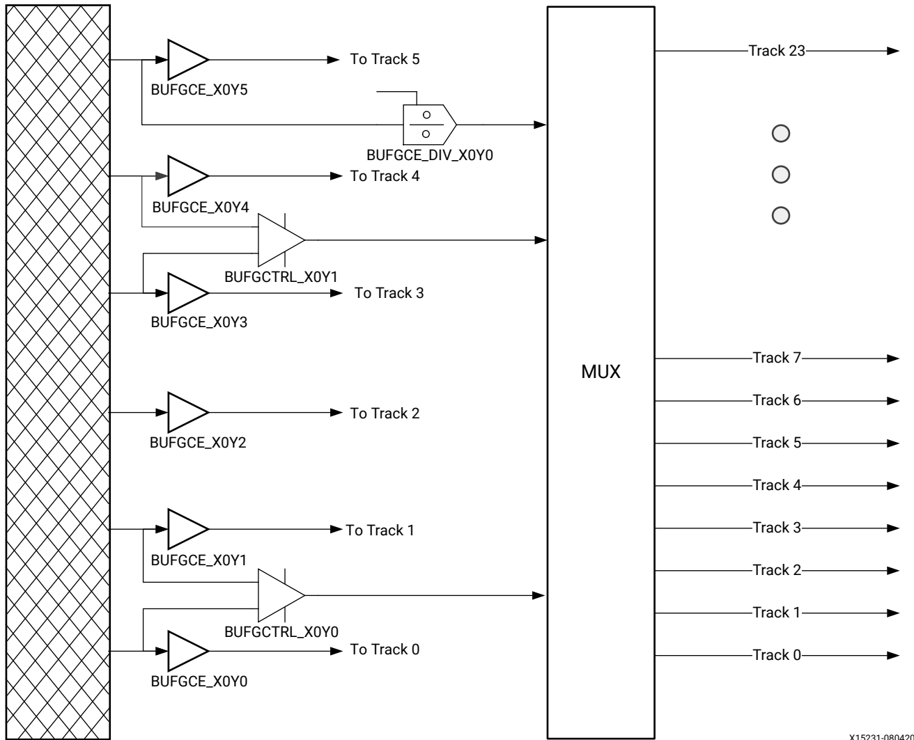
Figure 49: BUFGCE, BUFGCE_DIV, and BUFGCTRL Shared Inputs and Output Multiplexing
