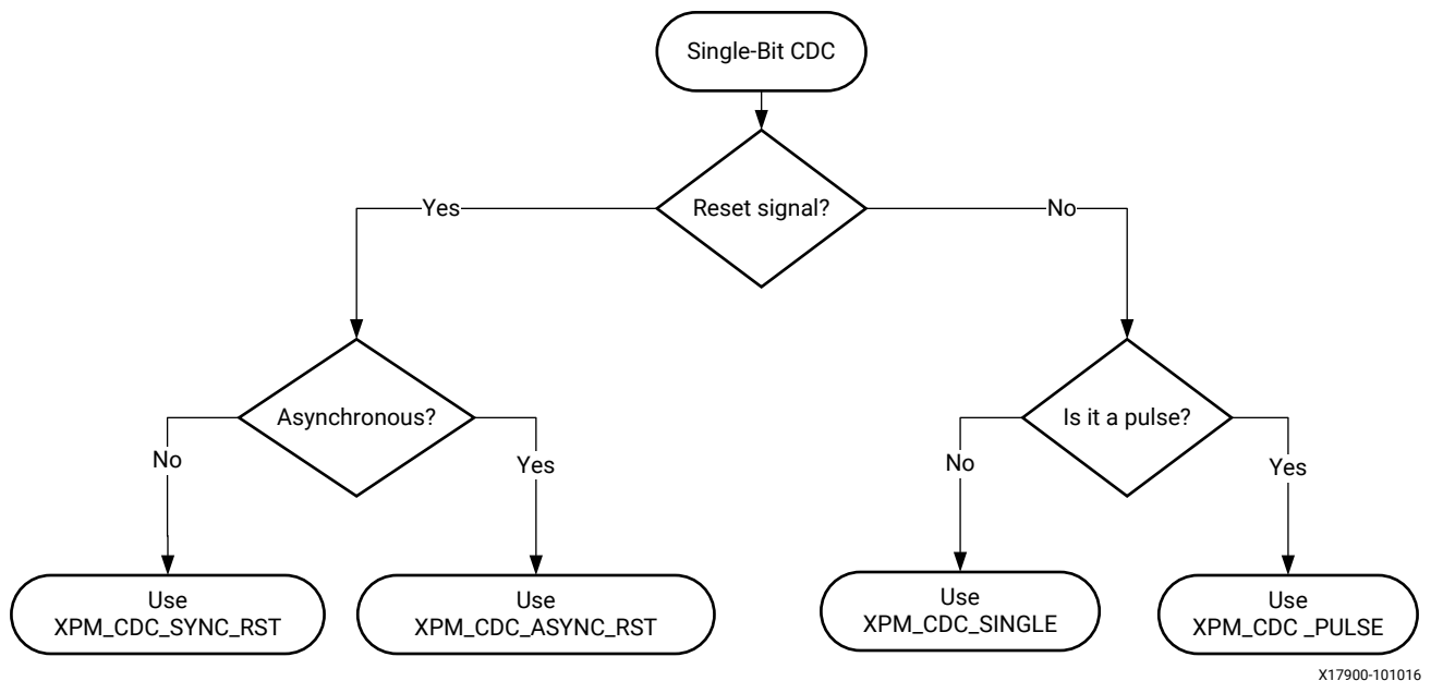
Figure 84: Single-Bit CDC Decision Tree
