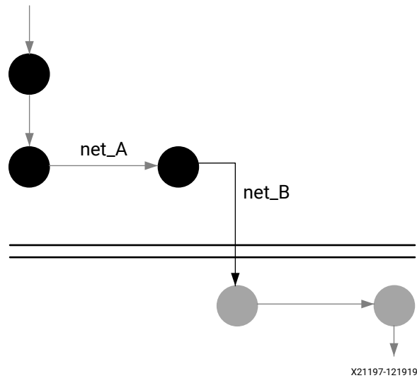
Figure 156: Optimal SLR Crossings After Setting the USER_CROSSING_SLR Property
