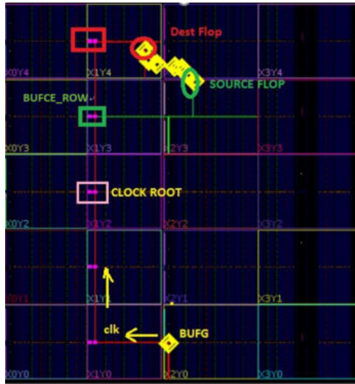
Figure 133: Clock Path from BUFG to the Leaf Level via BUFCE_ROW
