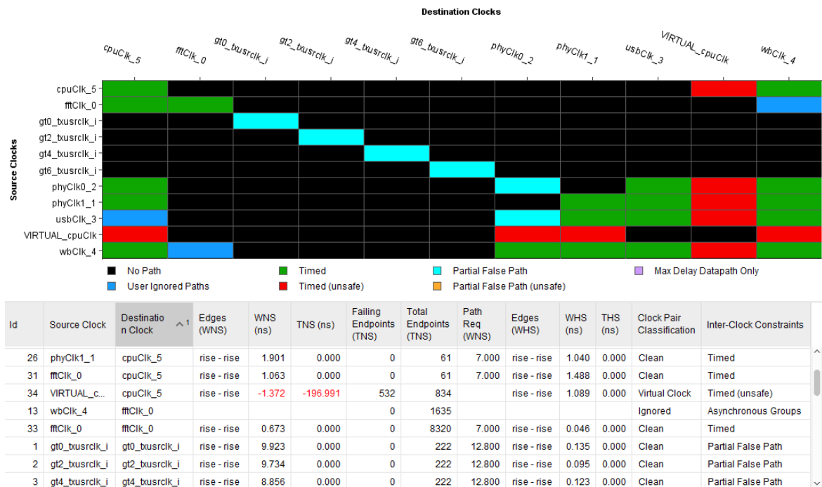
Figure 113: Sample Clock Interaction Report
