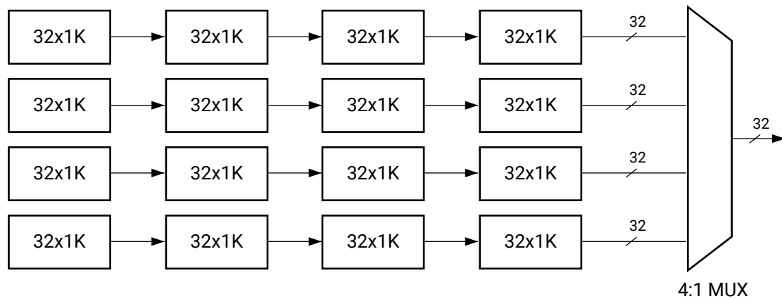
Figure 43: Generated Structure for 32x16K Memory Configuration Example Using CASCADE_HEIGHT and RAM_DECOMP Attributes
