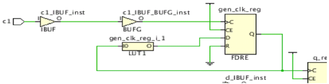
Figure 92: Generated Clock in the Fanout Of Master Clock
