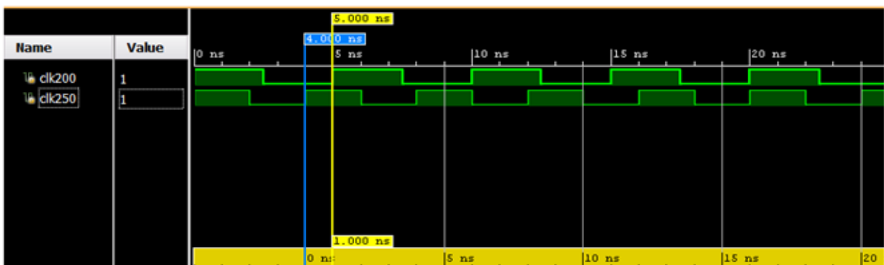
Figure 114: Clock Domain Crossing from 250 MHz to 200 MHz
