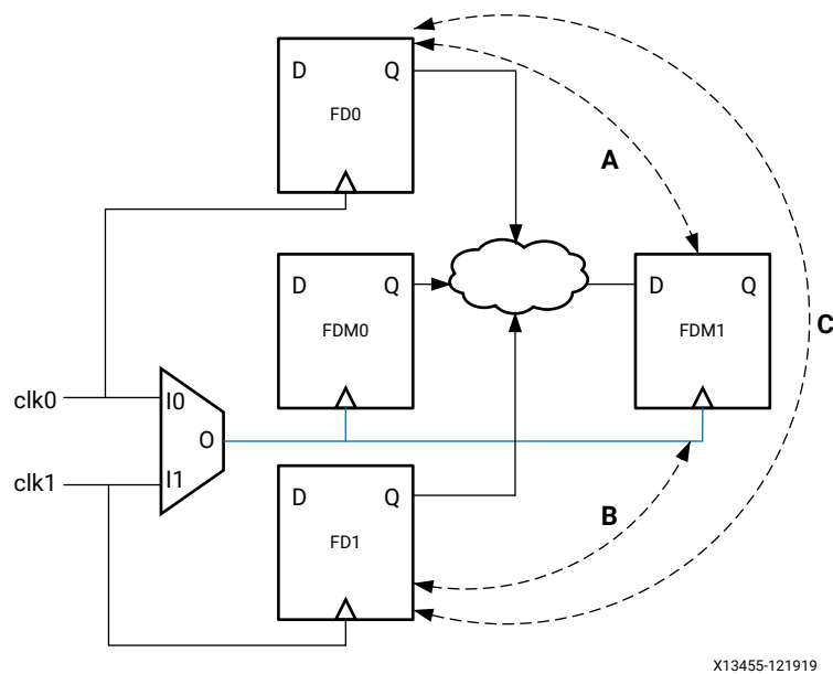
Figure 99: Multiplexed Clocks
