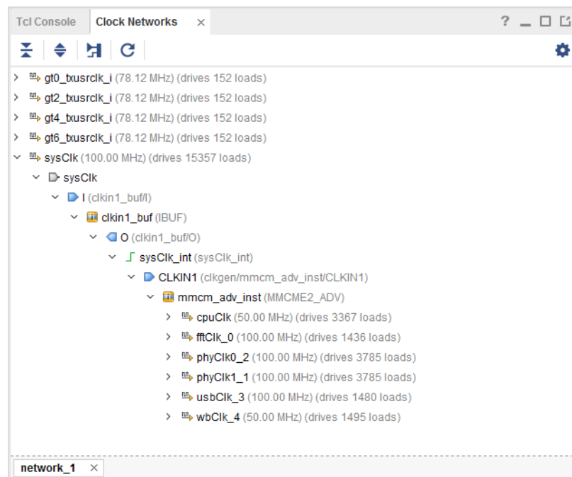
Figure 115: Report Clock Networks
