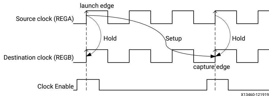
Figure 104: Setup/Hold Checks Modified After Multicycle Specification
