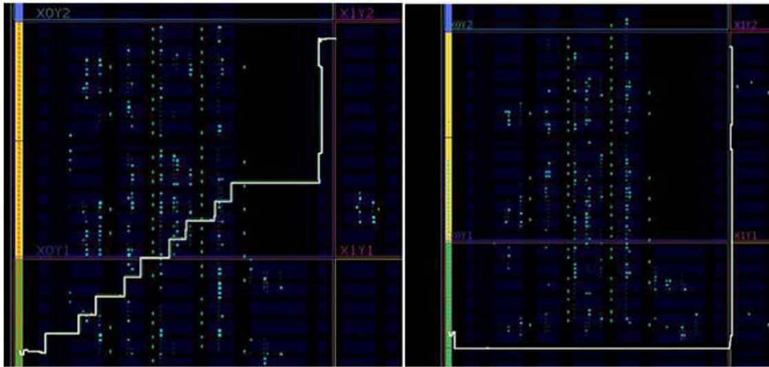
Figure 131: Comparison of Fabric Clock Route versus Dedicated Clock Route
