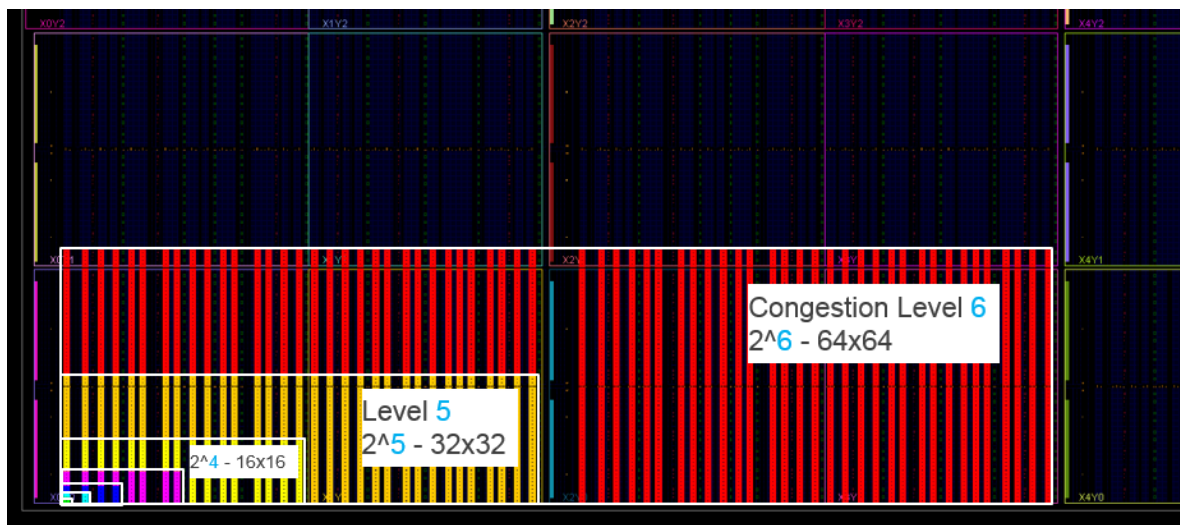
Figure 119: Congestion Levels and Areas in the Device View
