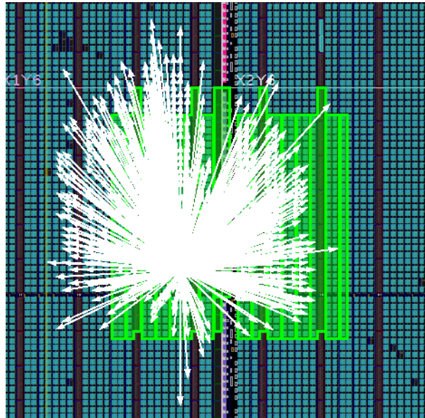
Figure 150: High-Fanout Nets in Congestion Window
