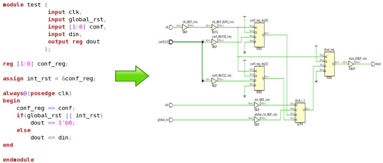
Figure 24: Multiple Reset Conditions Mapped Through Datapath Logic
