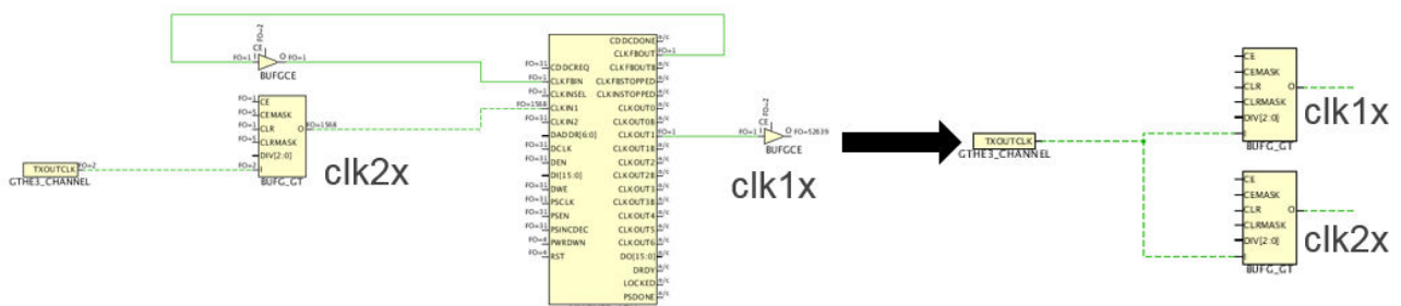
Figure 132: Implementing Balanced Clock Trees using UltraScale BUFG_GT
