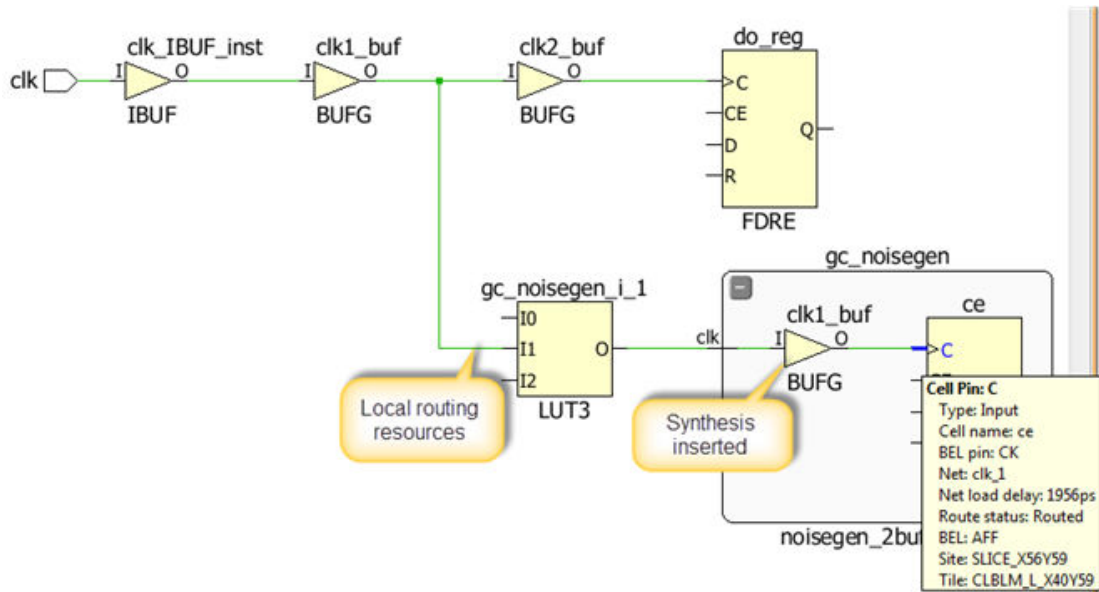
Figure 130: Skew Due to Local Routing on Clock Network
