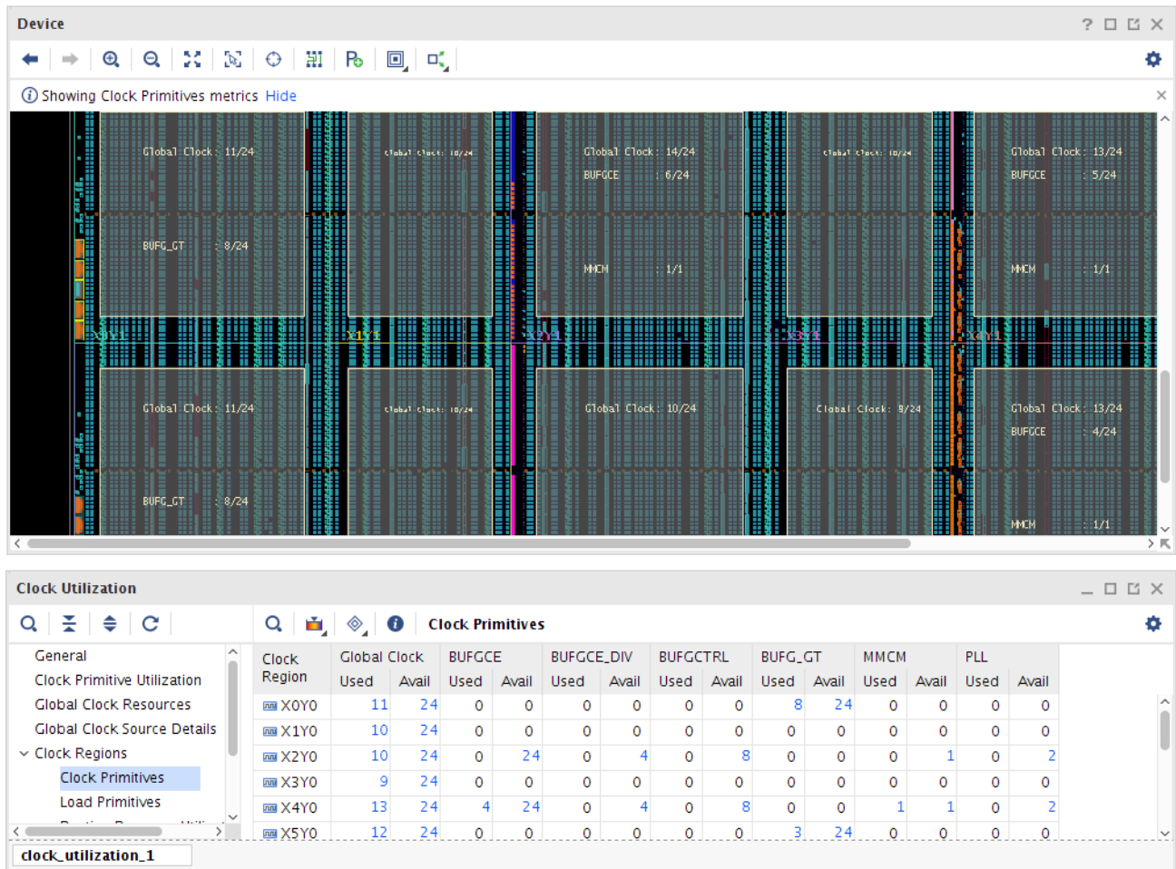
Figure 48: Clock Utilization Report
