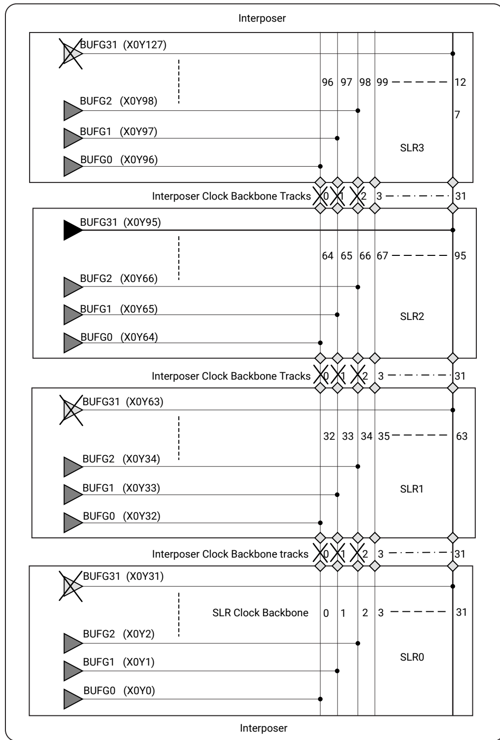
Figure 80: Optional Isolation on Clock Lines for SSI Devices
