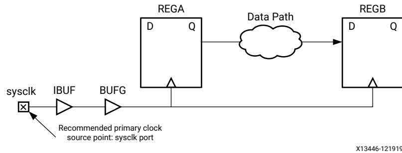
Figure 88: create_clock for Input Ports
