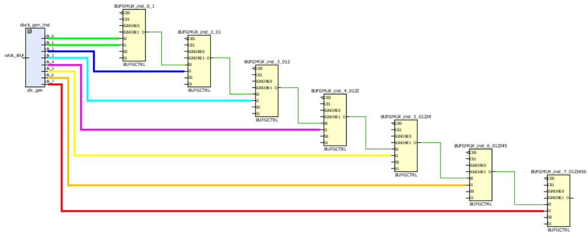
Figure 67: 8:1 MUX Using Cascaded BUFCTRL
