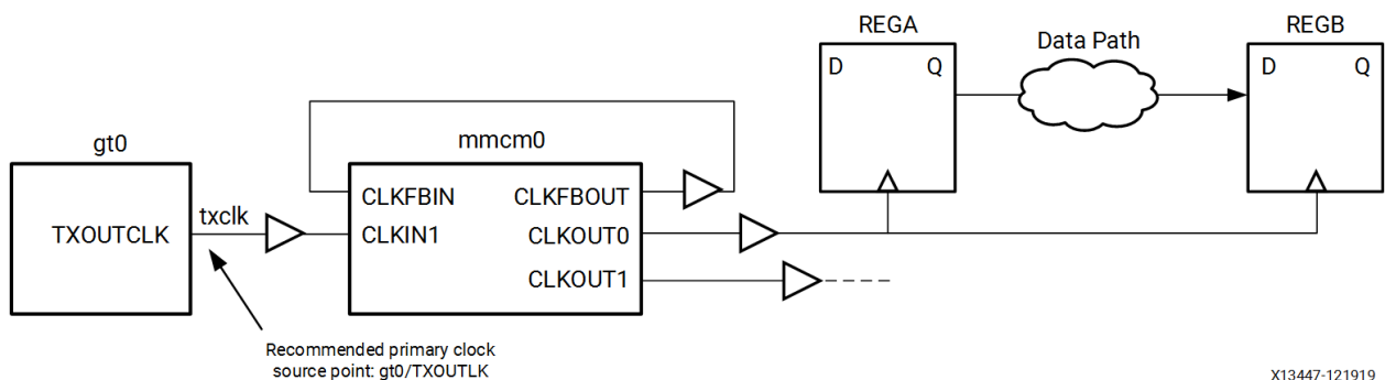
Figure 89: create_clock on a Primitive Pin
