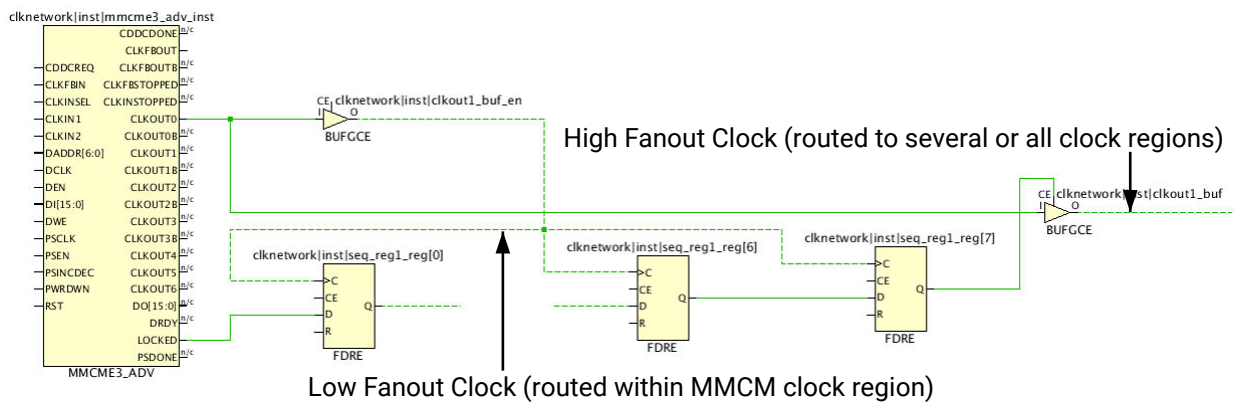
Figure 82: MMCM Safe Clock Startup Example
