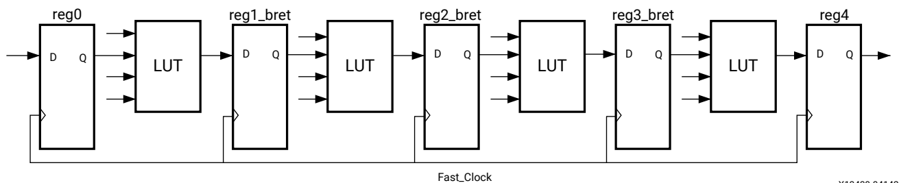
Figure 37: Pipelining After Retiming
