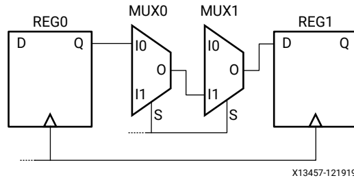
Figure 101: Path Cannot be Sensitized
