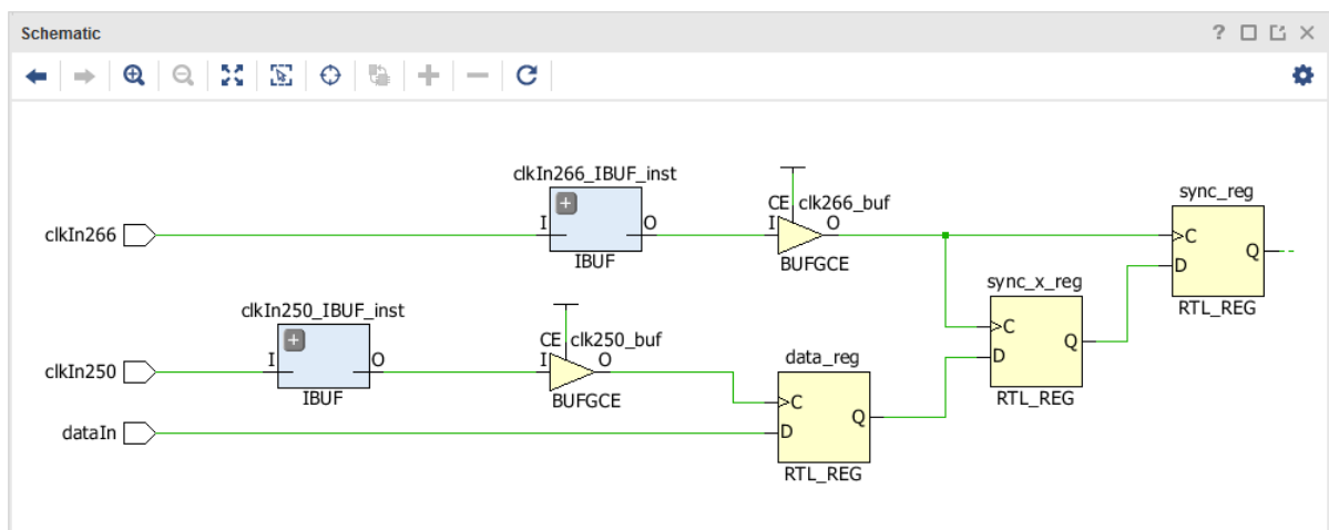
Figure 127: Asynchronous CDC Paths with Proper CDC Circuitry and No Common Node
