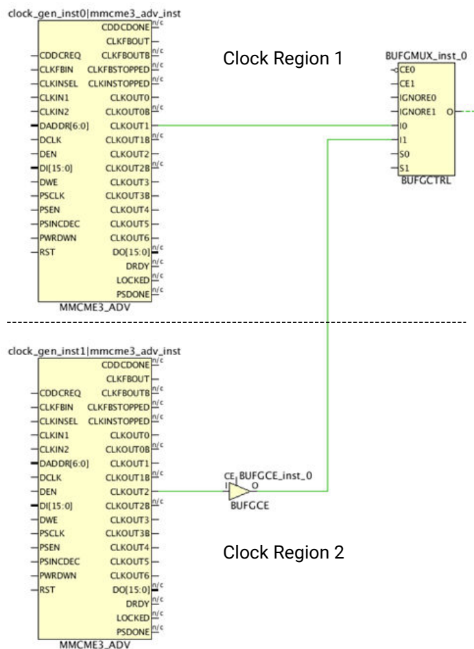
Figure 63: Routing the Clock to Another Clock Region
