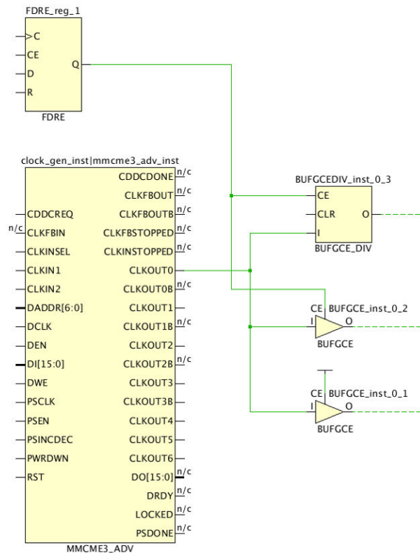
Figure 62: Parallel BUFGCE on MMCM Output
