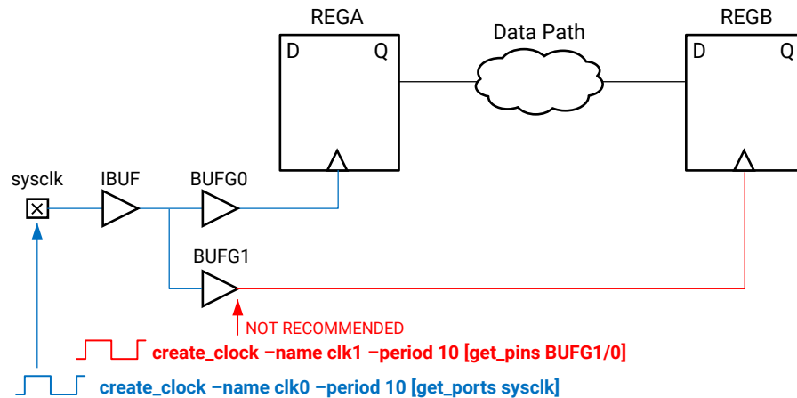
Figure 91: create_clock in the Fanout of Another Clock is Not Recommended
