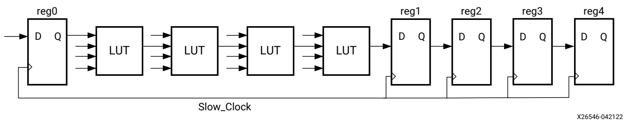
Figure 36: Pipelining After Adding Extra Registers
