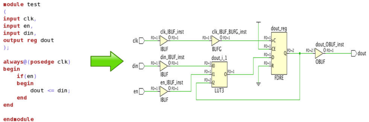
Figure 22: Clock Enable Implementation Using Datapath Logic
