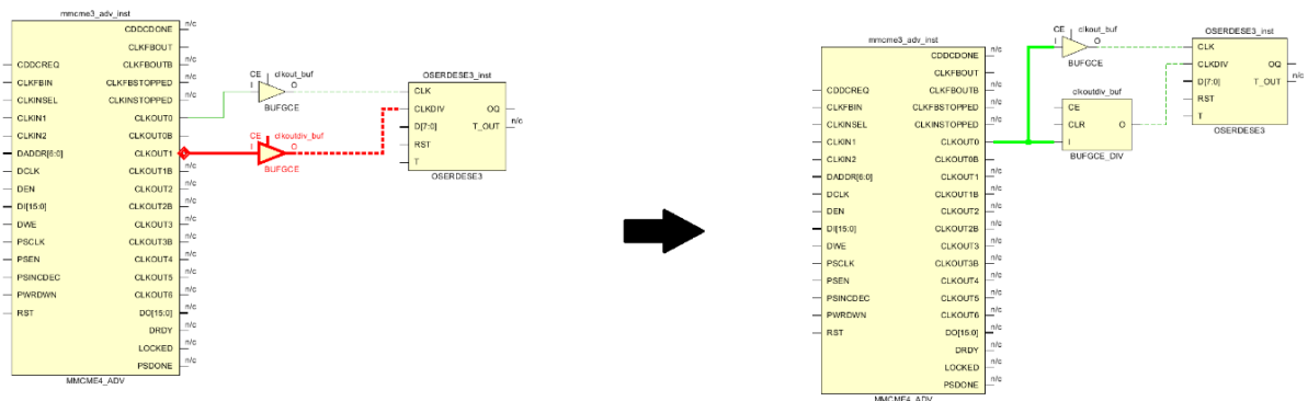
Figure 69: Suboptimal to Optimal Clocking Topologies for OSERDESE3
