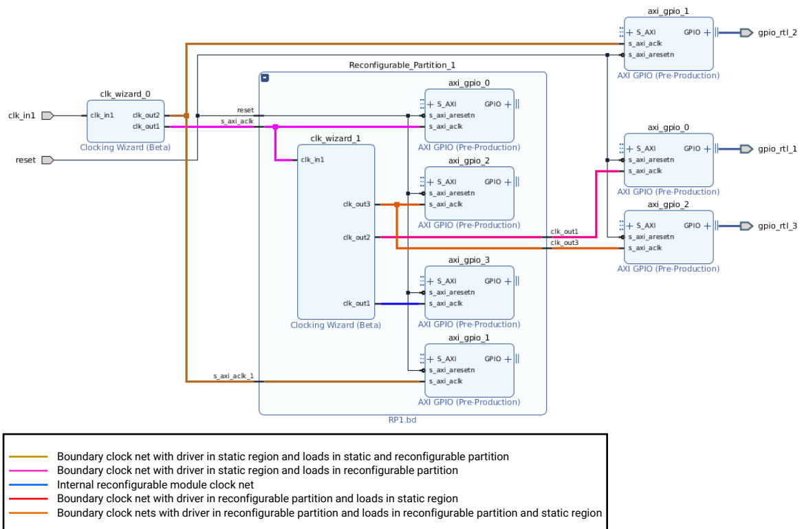
Figure 83: DFX Clock Tile Sharing
