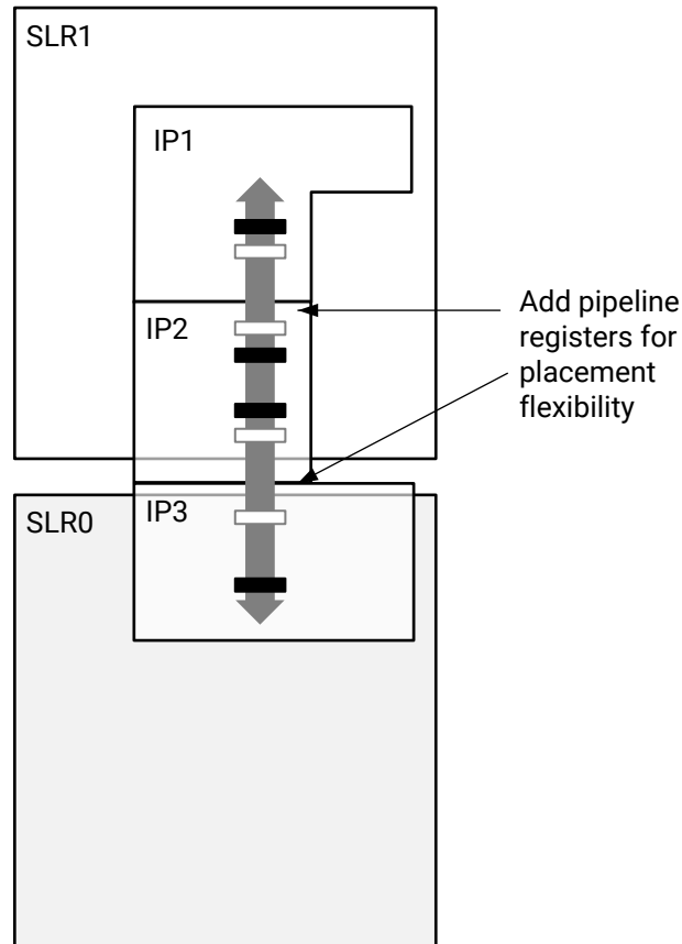
Figure 154: Placement Example for the USER_SLR_ASSIGNMENT Property
