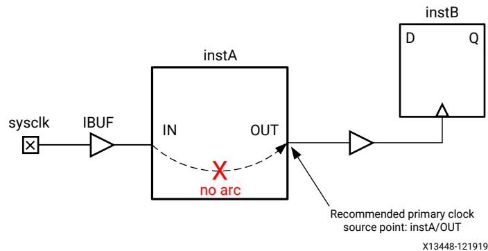
Figure 90: Clock Path Broken Due to a Missing Timing Arc
