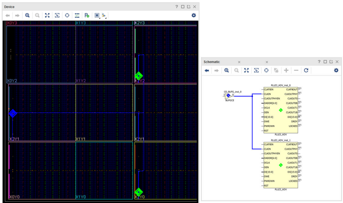
Figure 57: CLOCK_DEDICATED_ROUTE Set to ANY_CMT_COLUMN
