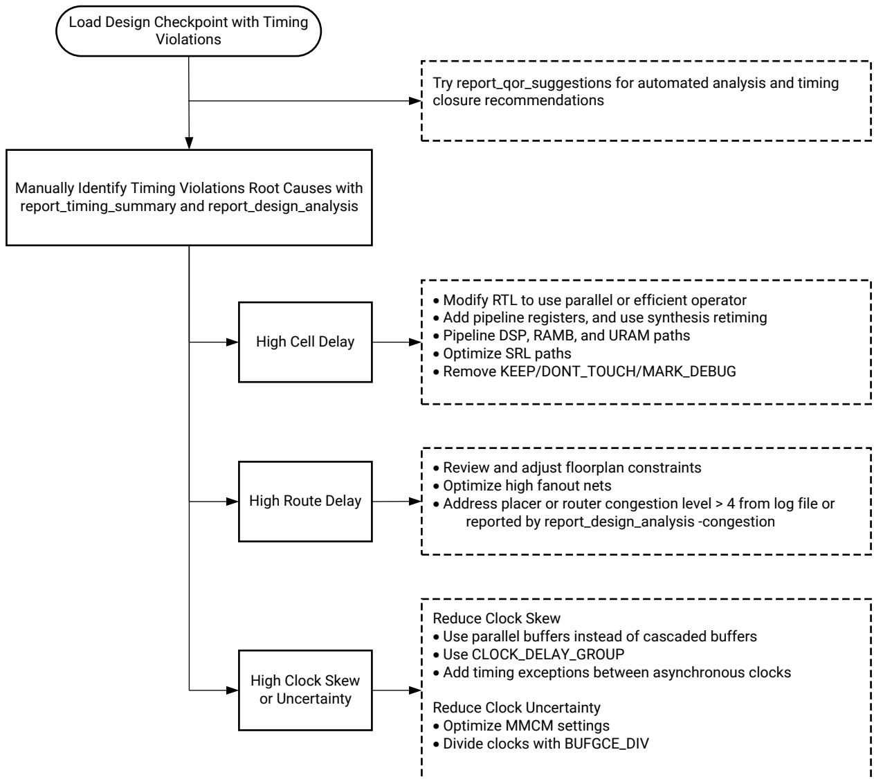
Figure 116: Analyzing and Resolving Timing Violations
