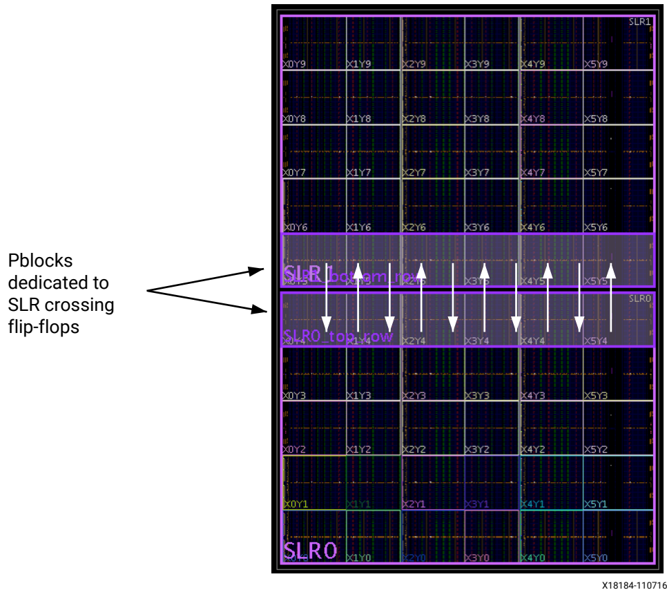
Figure 153: SLR-Crossing Pblock Example
