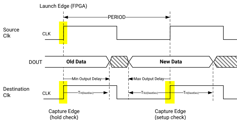
Figure 96: Interpreting Min and Max Output Delays
