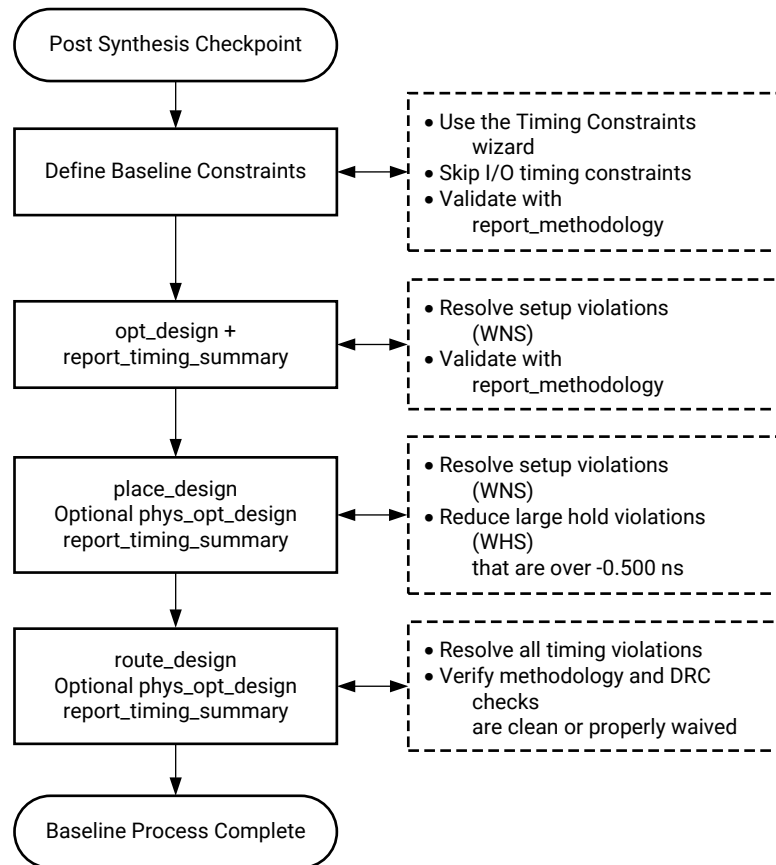
Figure 111: Baselining the Design
