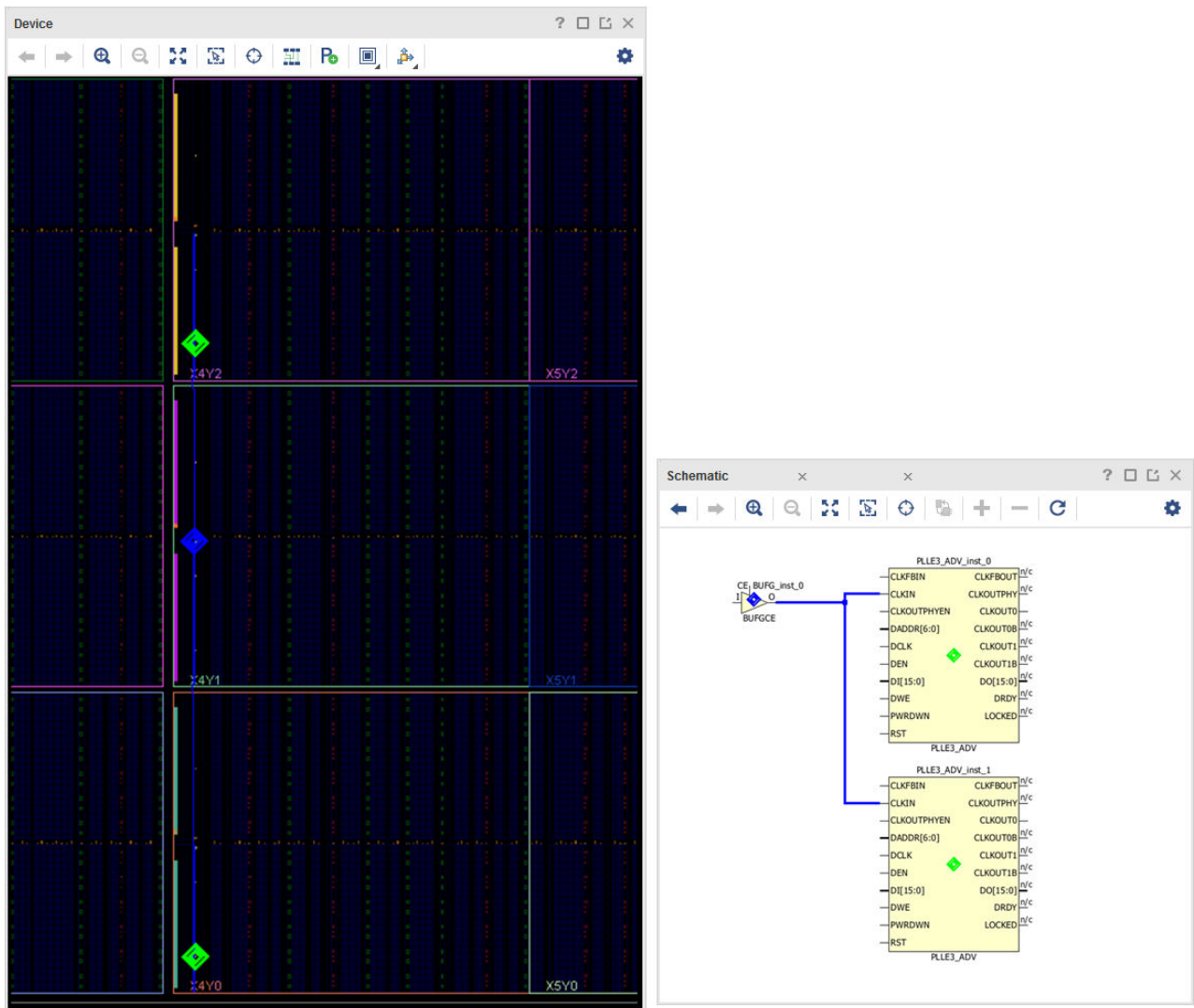
Figure 56: CLOCK_DEDICATED_ROUTE Constraint Set to SAME_CMT_COLUMN
