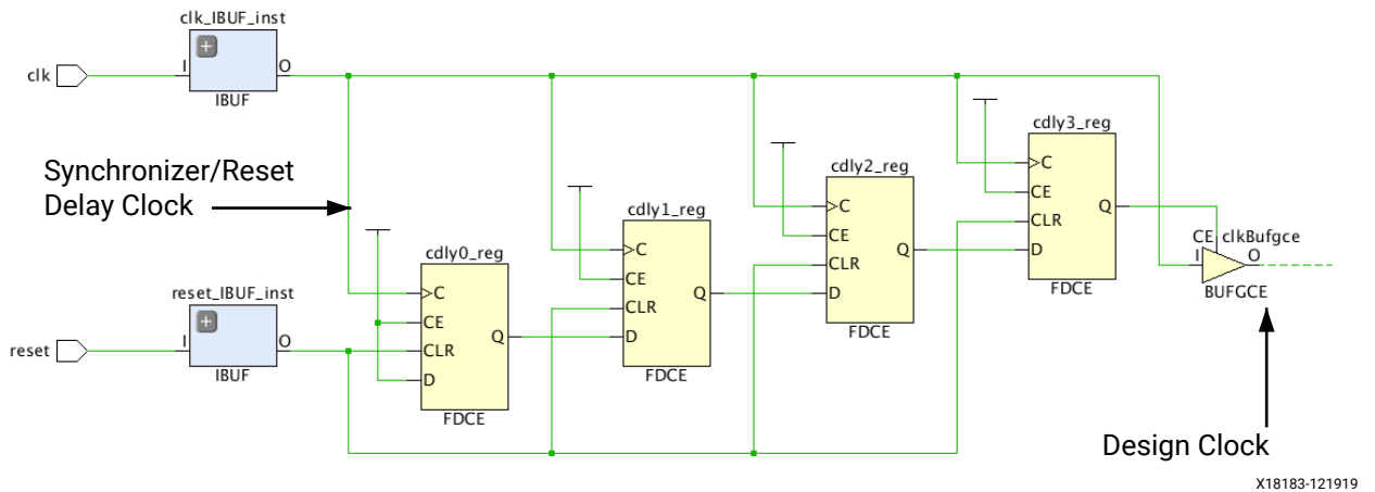
Figure 81: Reset Synchronization and Delay for Safe Clock Startup Example
