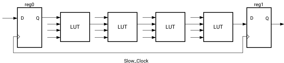
Figure 35: Before Pipelining
