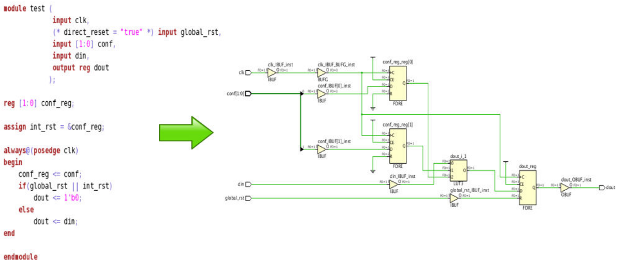
Figure 25: Dedicated Reset Pin Usage Using DIRECT_RESET Attribute
