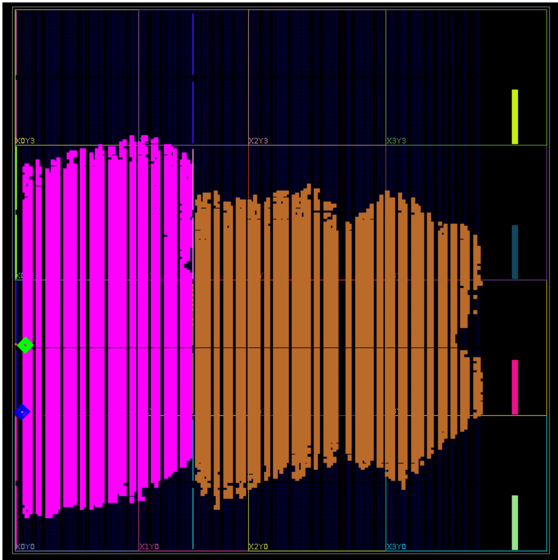
Figure 60: Fully Implemented Design with Placement of Clock Gating Synchronization Circuit
