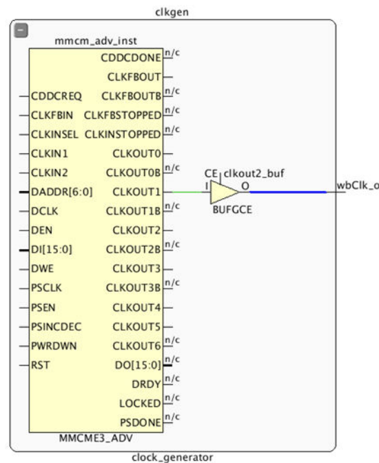
Figure 54: USER_CLOCK_ROOT Applied on the Net Segment Driven by the Clock Buffer
