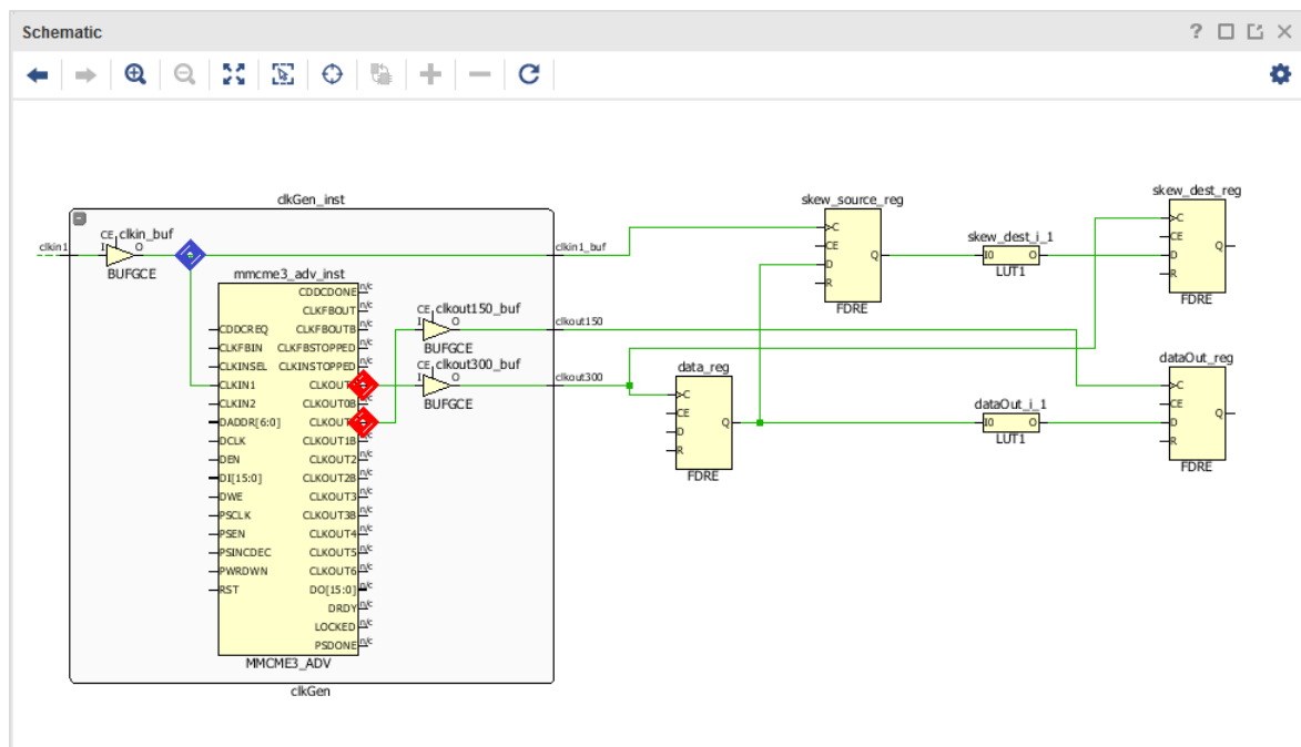
Figure 126: Synchronous CDC Paths with Common Nodes on Input and Output of a MMCM
