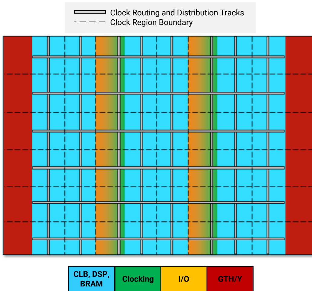
Figure 47: UltraScale Device Clock Region Tiles
