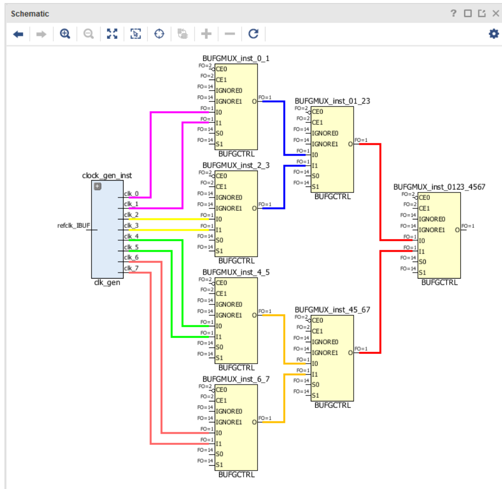
Figure 66: Non-Recommended 8:1 Balanced Clock MUX Structure
