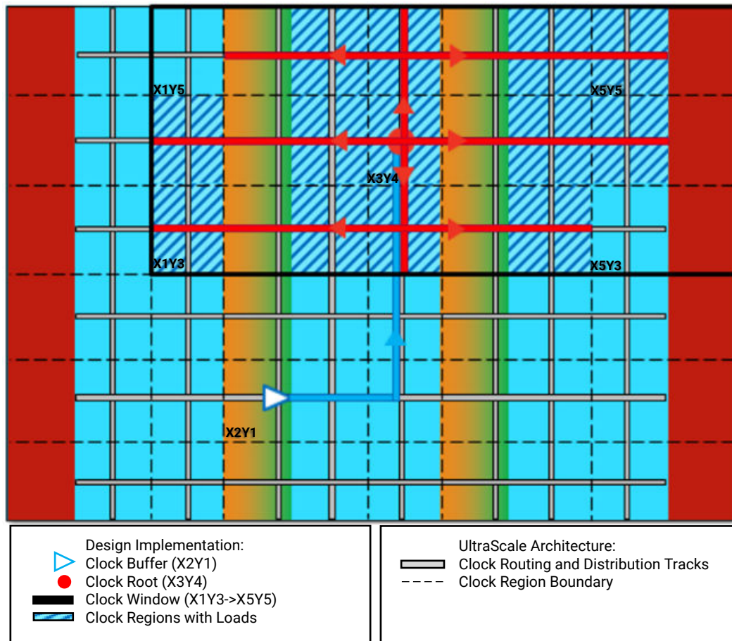
Figure 50: UltraScale Device Clock Routing from Driver to Loads
