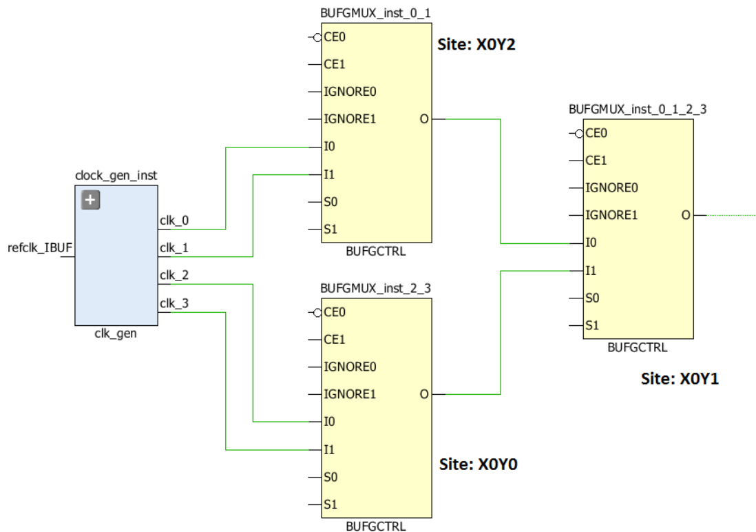
Figure 65: 4:1 MUX Using Parallel BUFGCTRL
