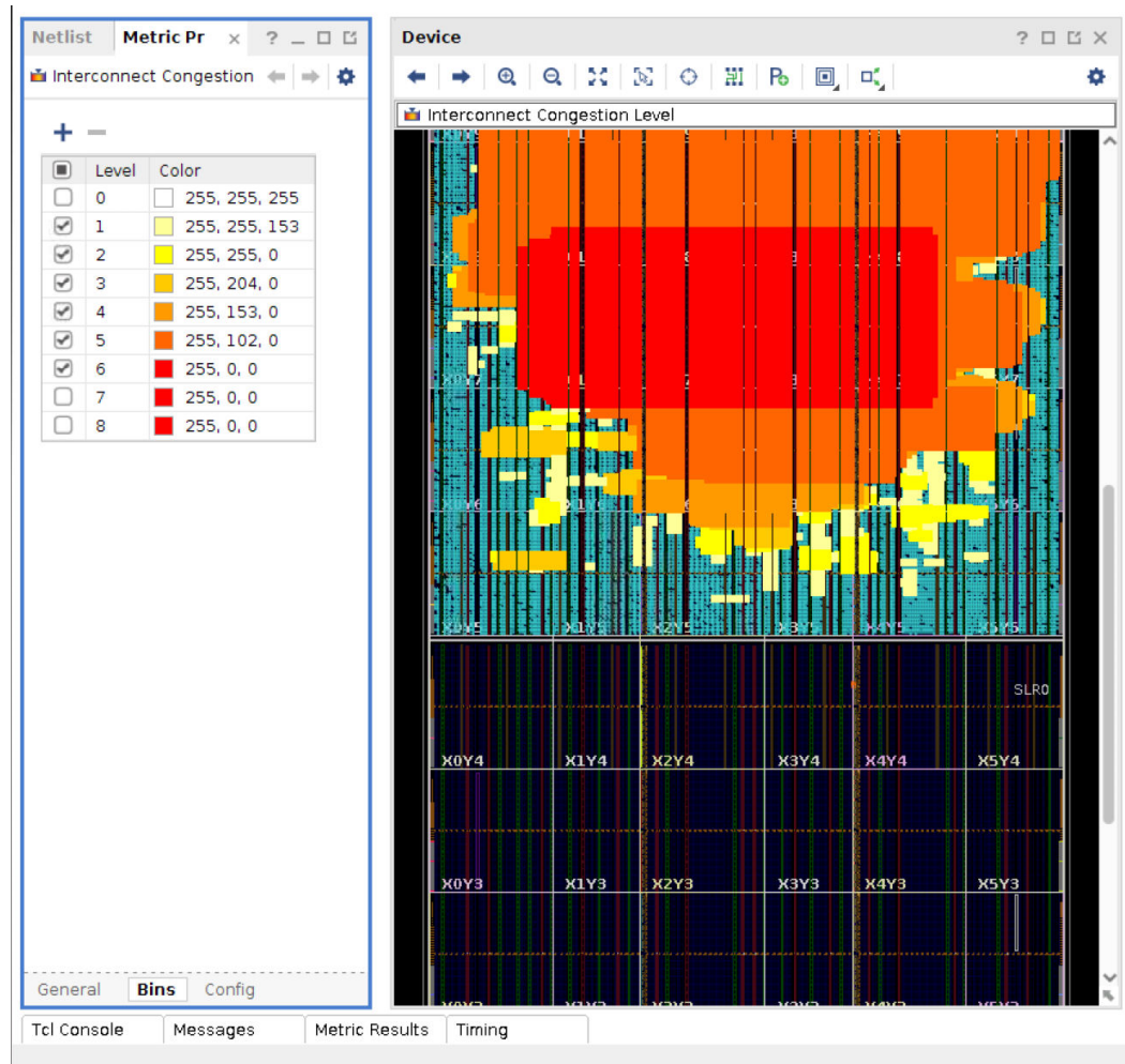
Figure 144: Utilization Analysis per SLR Region
