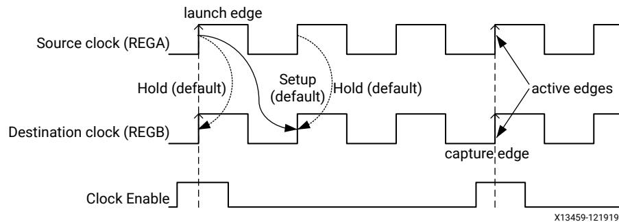
Figure 103: Timing Diagram for Setup/Hold Check
