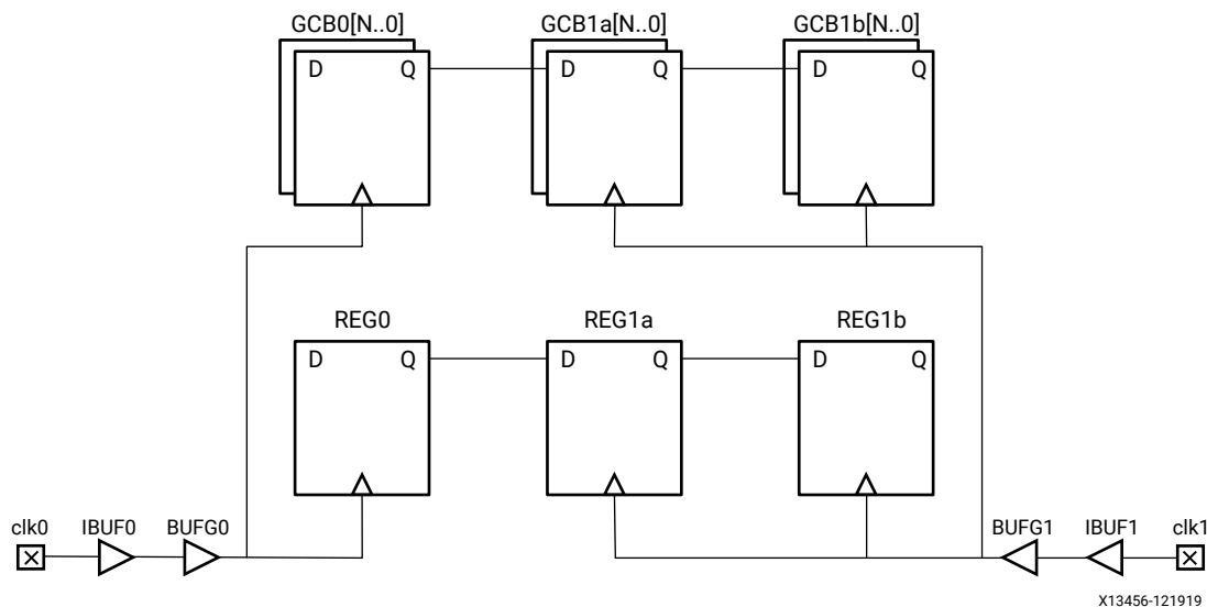
Figure 100: Multiple Interactions Between Two Asynchronous Clocks
