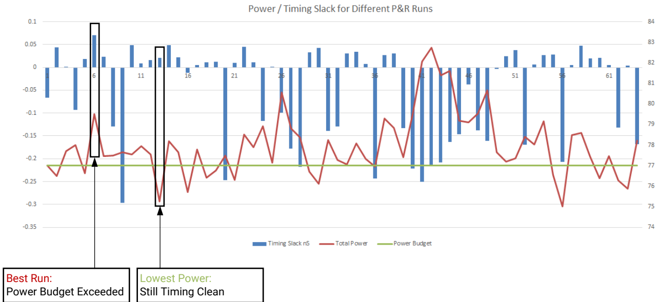
Figure 158: Power and Timing Slack for Different Place and Route Runs
