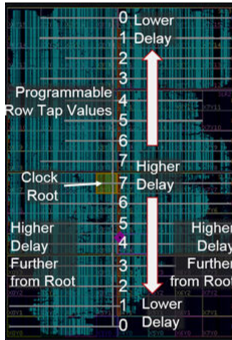
Figure 134: Row Programmable Tap Delay Settings Across an UltraScale+ SSI Technology Device
