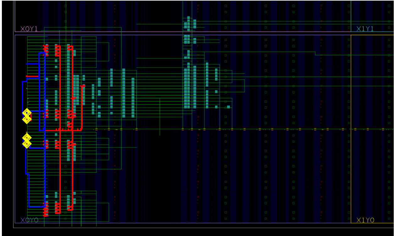
Figure 78: TXUSRCLK/TXUSRCLK2 Clock Routing for a Single-Quad Interface
