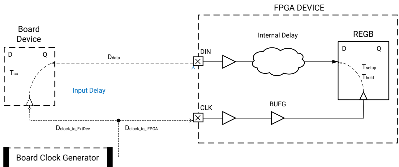
Figure 93: Input Delay Computation
