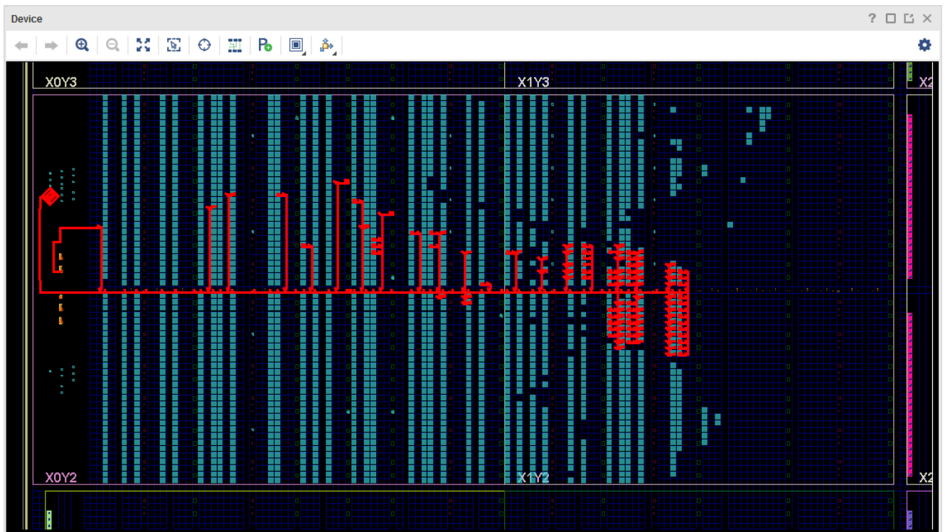
Figure 53: Low Fanout Clock Contained in Two Clock Regions
