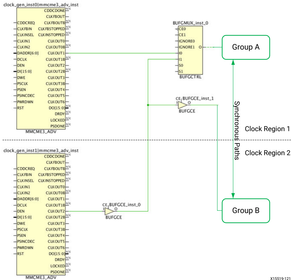
Figure 64: Balancing Clock Trees for Synchronous Paths Between Clock Regions
