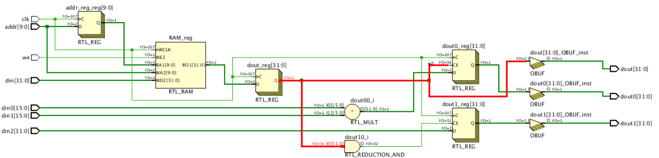
Figure 30: Multiple Fanout Preventing Block RAM Output Register Inference
