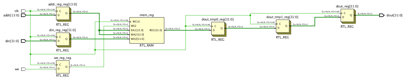
Figure 42: 32x16K Memory Configuration
