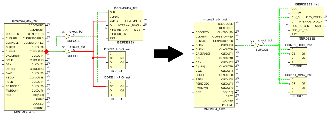
Figure 68: Suboptimal to Optimal Clocking Topologies for ISERDESE3 and IDDRE1
