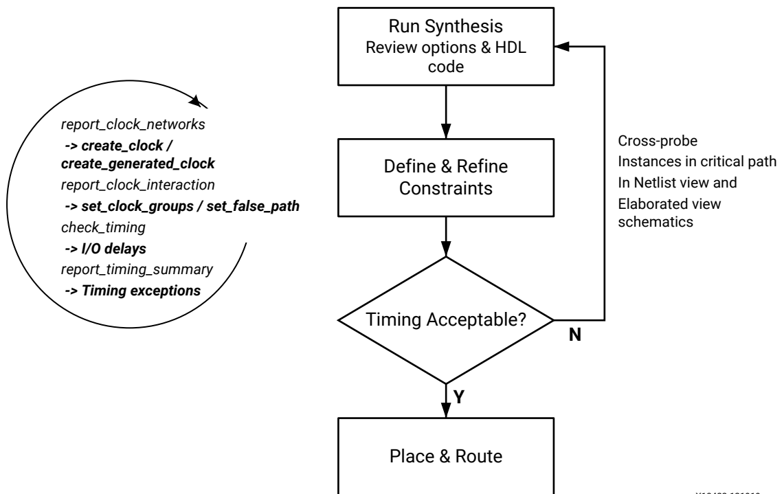
Figure 110: Design Methodology for Rapid Convergence
